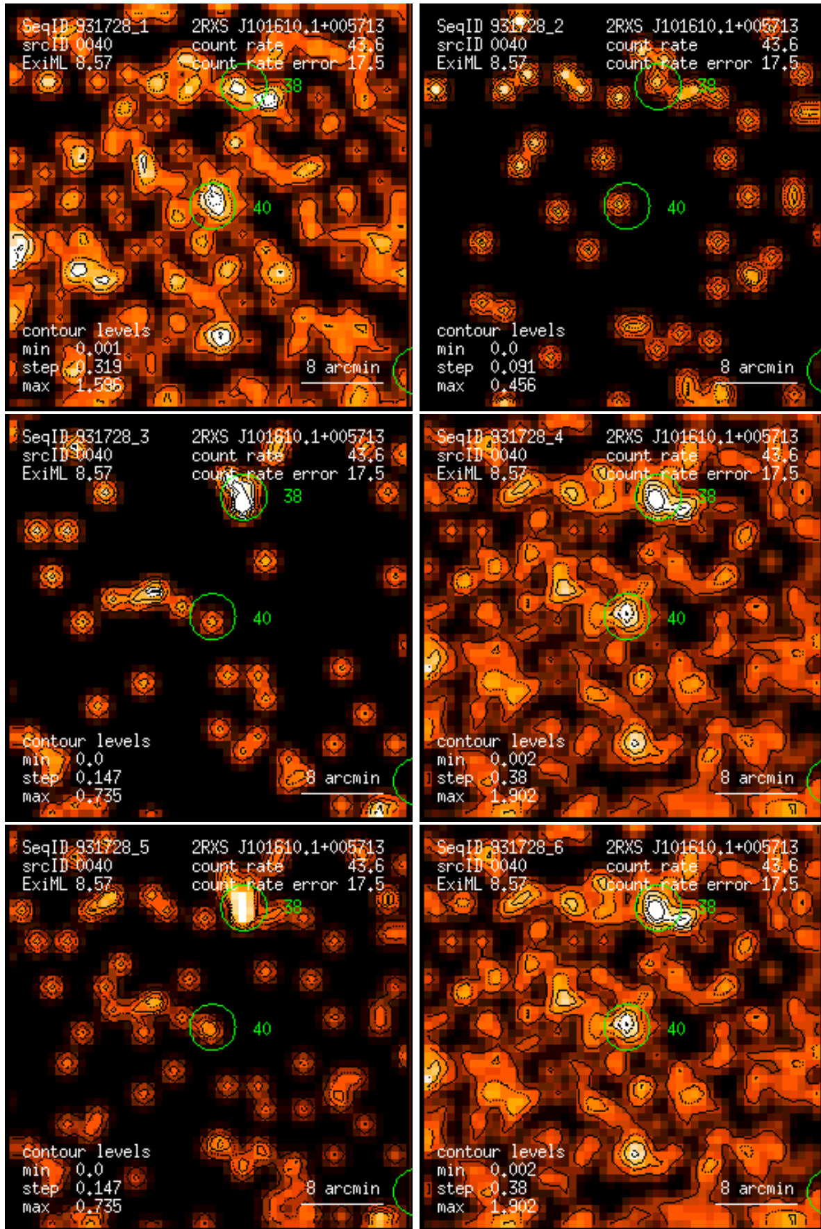
Figure 40: RASS 931728: detection 0040: band rate images, Gaussian filter: (1) PSPC channels 11 – 41, (2) 52 – 90, (3) 91 – 201, (4) 11 – 235, (5) 52 – 201, (6) 11 – 201. Broad band rates in counts/ks. Band rate contour levels in counts/ks/arcmin 2 .
