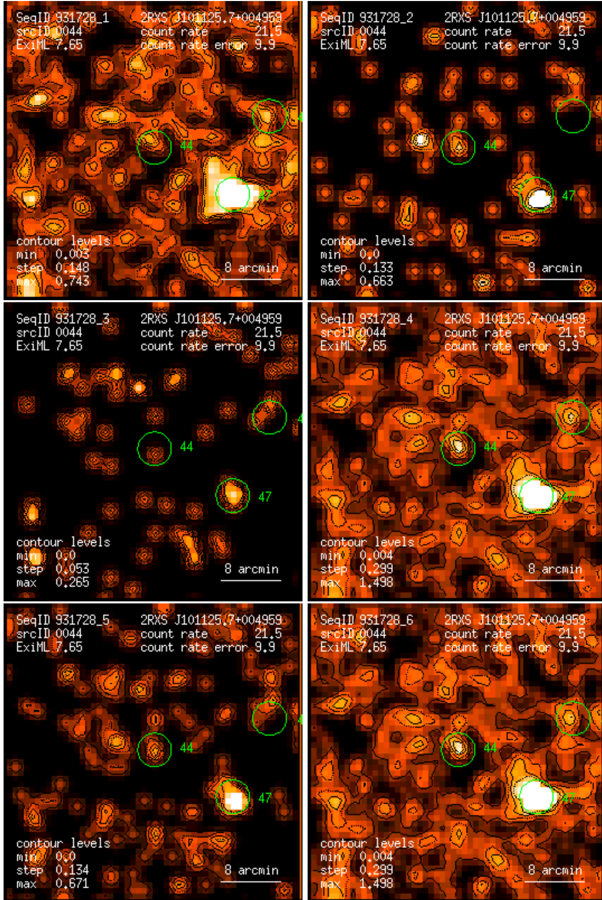
Figure 44: RASS 931728: detection 0044: band rate images, Gaussian filter: (1) PSPC channels 11 – 41, (2) 52 – 90, (3) 91 – 201, (4) 11 – 235, (5) 52 – 201, (6) 11 – 201. Broad band rates in counts/ks. Band rate contour levels in counts/ks/arcmin 2 .
