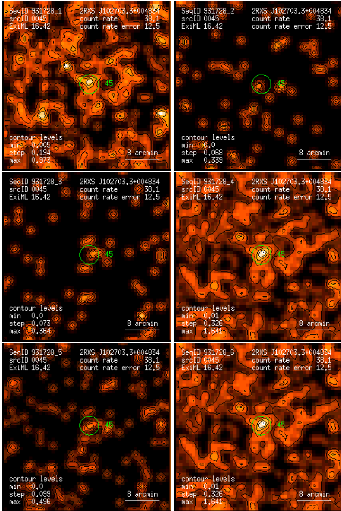
Figure 45: RASS 931728: detection 0045: band rate images, Gaussian filter: (1) PSPC channels 11 – 41, (2) 52 – 90, (3) 91 – 201, (4) 11 – 235, (5) 52 – 201, (6) 11 – 201. Broad band rates in counts/ks. Band rate contour levels in counts/ks/arcmin 2 .
