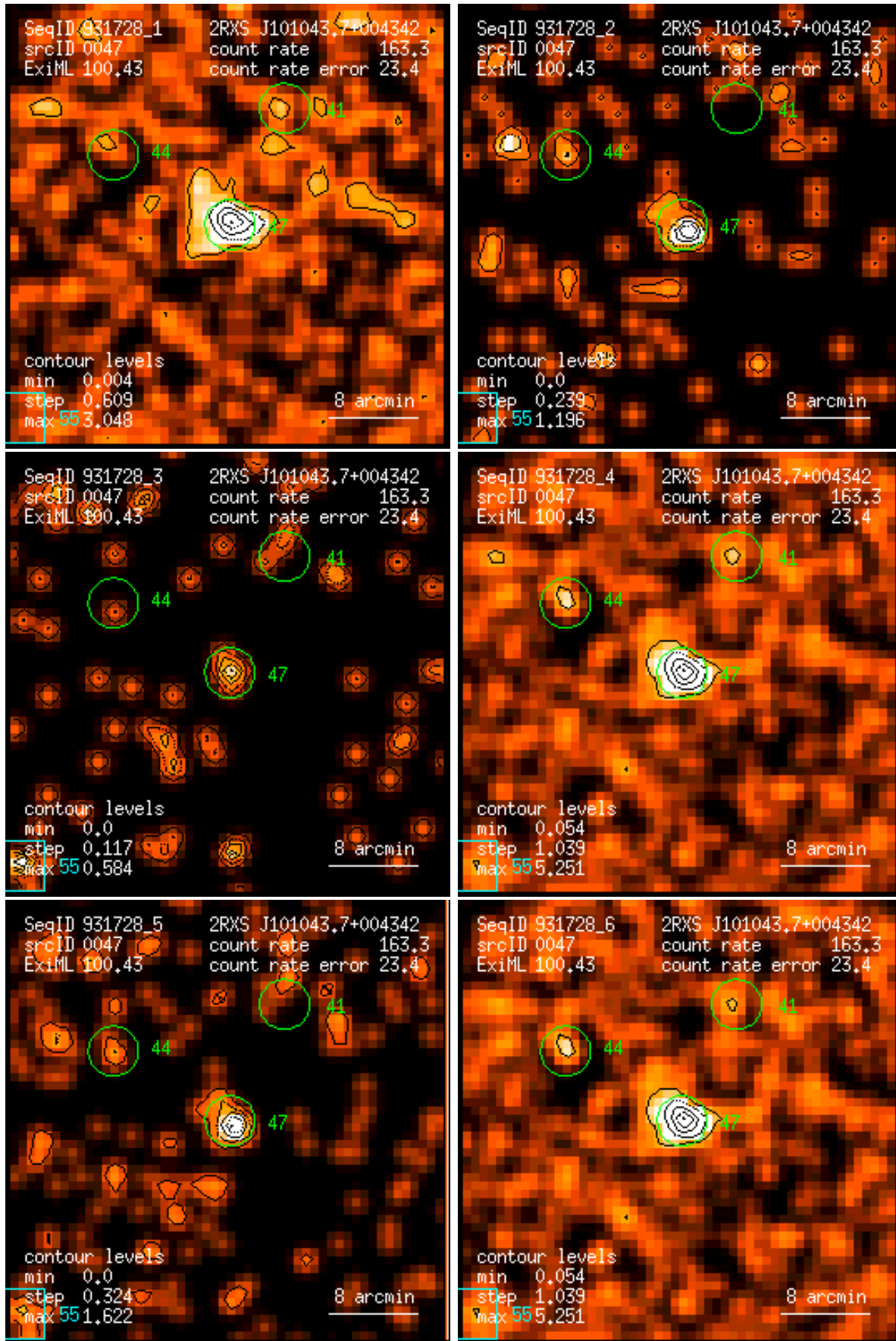
Figure 47: RASS 931728: detection 0047: band rate images, Gaussian filter: (1) PSPC channels 11 – 41, (2) 52 – 90, (3) 91 – 201, (4) 11 – 235, (5) 52 – 201, (6) 11 – 201. Broad band rates in counts/ks. Band rate contour levels in counts/ks/arcmin 2 .
