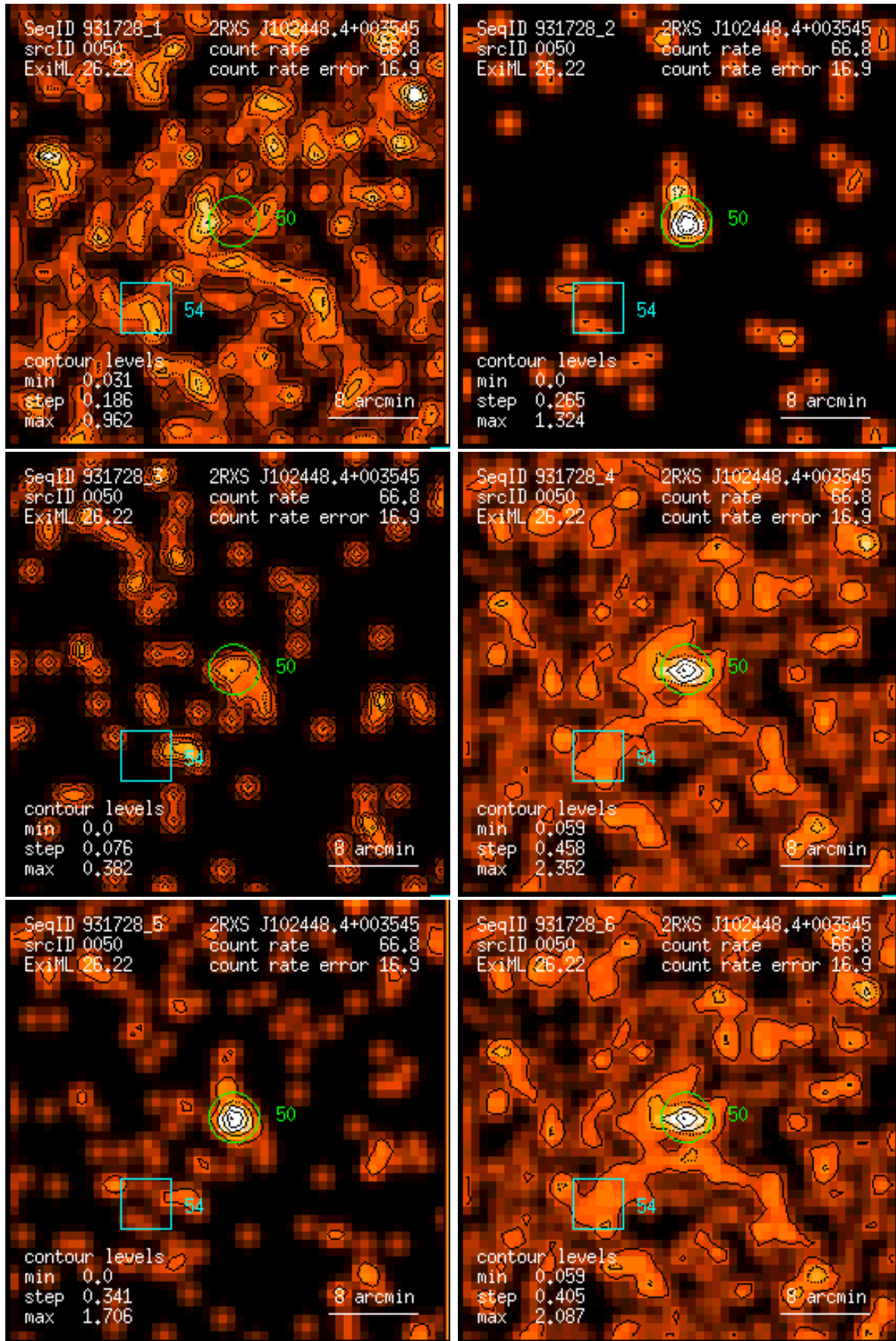
Figure 50: RASS 931728: detection 0050: band rate images, Gaussian filter: (1) PSPC channels 11 – 41, (2) 52 – 90, (3) 91 – 201, (4) 11 – 235, (5) 52 – 201, (6) 11 – 201. Broad band rates in counts/ks. Band rate contour levels in counts/ks/arcmin 2 .
