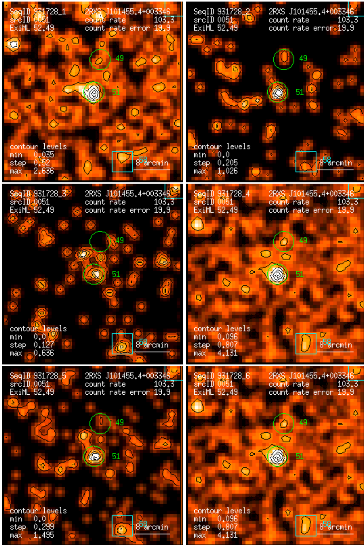
Figure 51: RASS 931728: detection 0051: band rate images, Gaussian filter: (1) PSPC channels 11 – 41, (2) 52 – 90, (3) 91 – 201, (4) 11 – 235, (5) 52 – 201, (6) 11 – 201. Broad band rates in counts/ks. Band rate contour levels in counts/ks/arcmin 2 .
