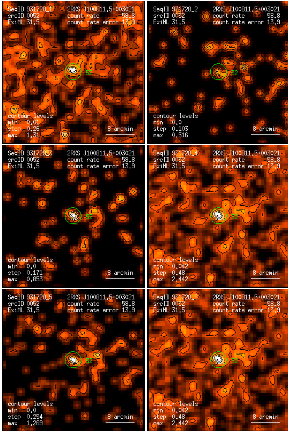
Figure 52: RASS 931728: detection 0052: band rate images, Gaussian filter: (1) PSPC channels 11 – 41, (2) 52 – 90, (3) 91 – 201, (4) 11 – 235, (5) 52 – 201, (6) 11 – 201. Broad band rates in counts/ks. Band rate contour levels in counts/ks/arcmin 2 .
