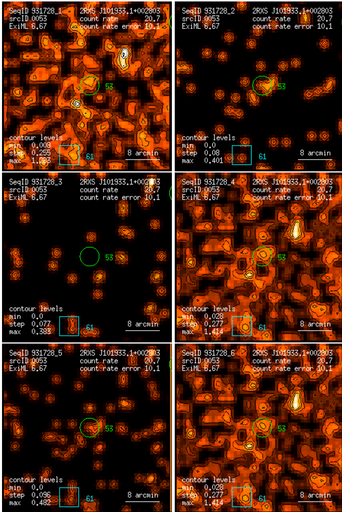
Figure 53: RASS 931728: detection 0053: band rate images, Gaussian filter: (1) PSPC channels 11 – 41, (2) 52 – 90, (3) 91 – 201, (4) 11 – 235, (5) 52 – 201, (6) 11 – 201. Broad band rates in counts/ks. Band rate contour levels in counts/ks/arcmin 2 .
