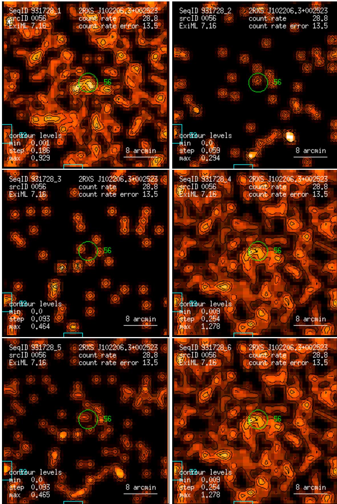
Figure 56: RASS 931728: detection 0056: band rate images, Gaussian filter: (1) PSPC channels 11 – 41, (2) 52 – 90, (3) 91 – 201, (4) 11 – 235, (5) 52 – 201, (6) 11 – 201. Broad band rates in counts/ks. Band rate contour levels in counts/ks/arcmin 2 .
