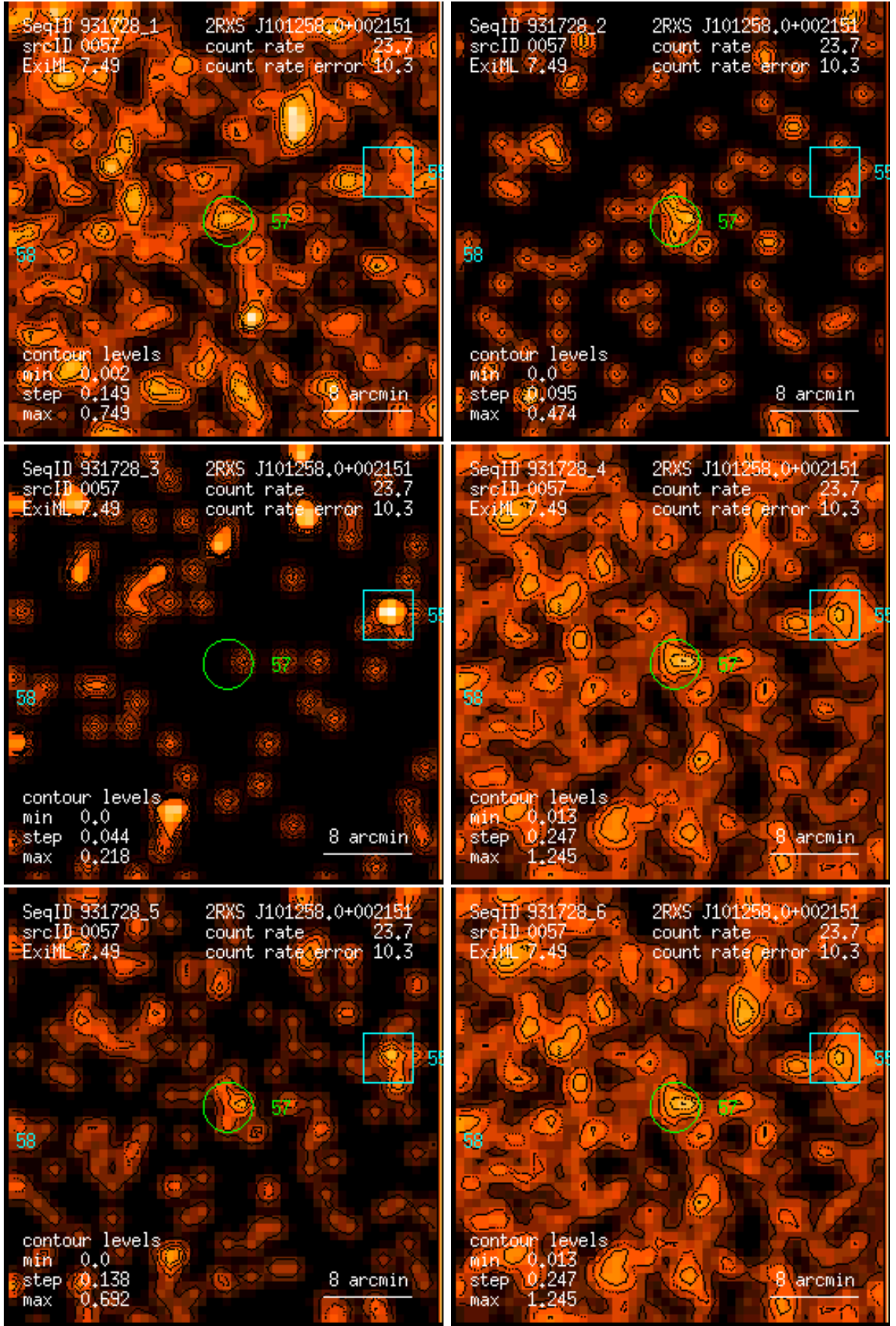
Figure 57: RASS 931728: detection 0057: band rate images, Gaussian filter: (1) PSPC channels 11 – 41, (2) 52 – 90, (3) 91 – 201, (4) 11 – 235, (5) 52 – 201, (6) 11 – 201. Broad band rates in counts/ks. Band rate contour levels in counts/ks/arcmin 2 .
