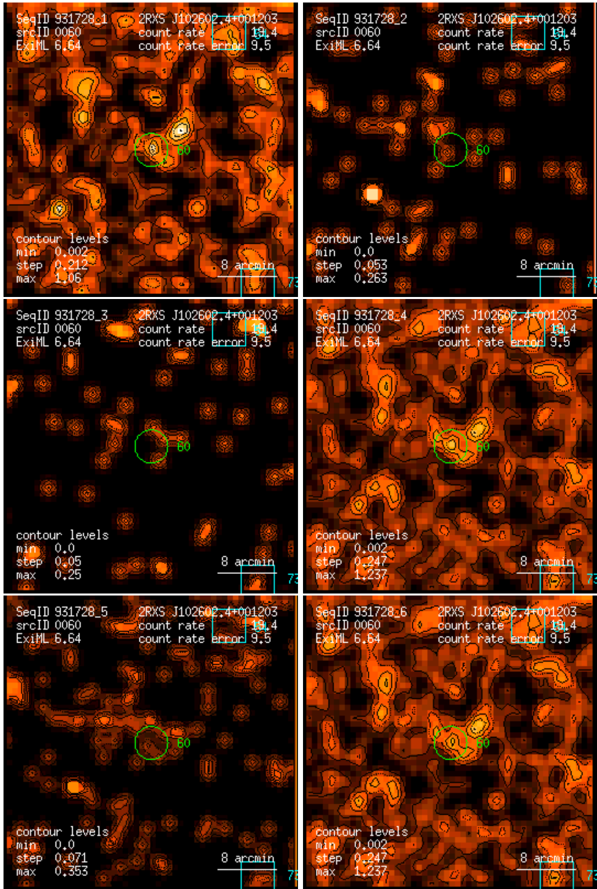
Figure 60: RASS 931728: detection 0060: band rate images, Gaussian filter: (1) PSPC channels 11 – 41, (2) 52 – 90, (3) 91 – 201, (4) 11 – 235, (5) 52 – 201, (6) 11 – 201. Broad band rates in counts/ks. Band rate contour levels in counts/ks/arcmin 2 .
