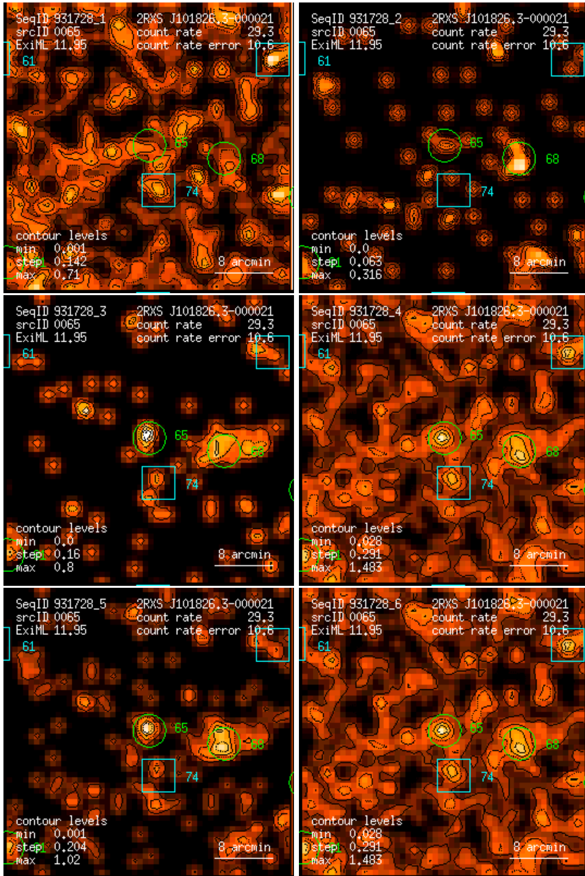
Figure 65: RASS 931728: detection 0065: band rate images, Gaussian filter: (1) PSPC channels 11 – 41, (2) 52 – 90, (3) 91 – 201, (4) 11 – 235, (5) 52 – 201, (6) 11 – 201. Broad band rates in counts/ks. Band rate contour levels in counts/ks/arcmin 2 .
