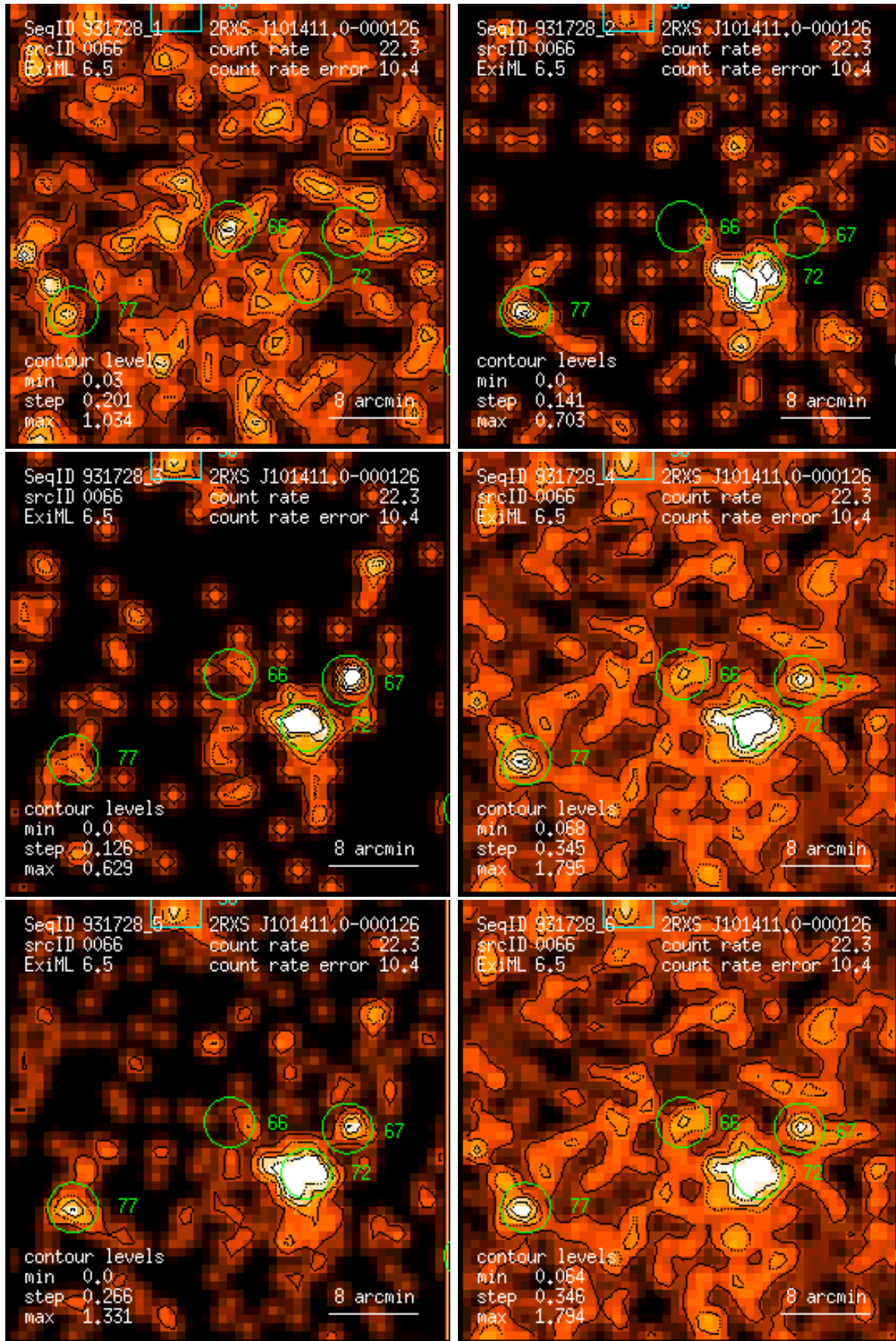
Figure 66: RASS 931728: detection 0066: band rate images, Gaussian filter: (1) PSPC channels 11 – 41, (2) 52 – 90, (3) 91 – 201, (4) 11 – 235, (5) 52 – 201, (6) 11 – 201. Broad band rates in counts/ks. Band rate contour levels in counts/ks/arcmin 2 .
