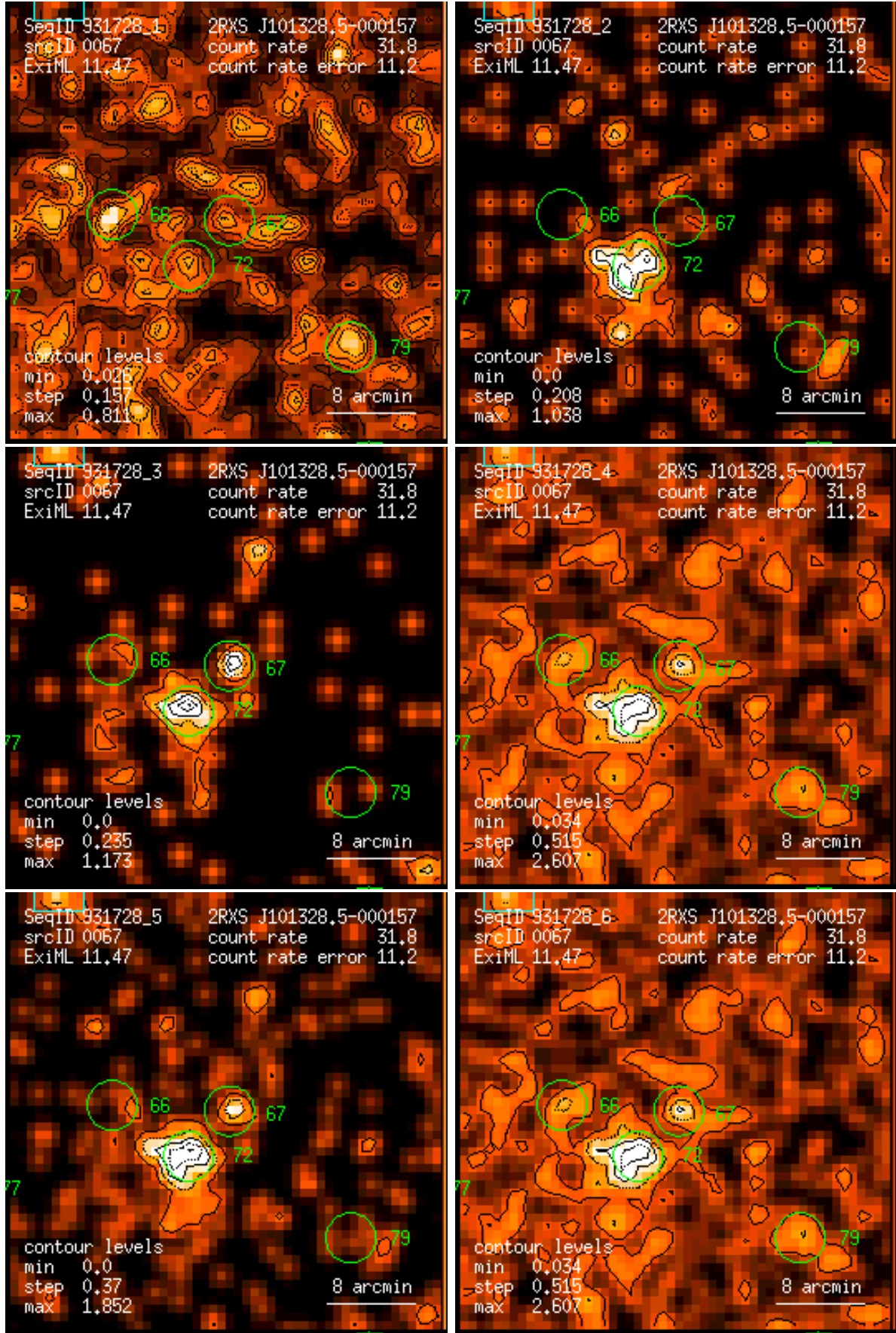
Figure 67: RASS 931728: detection 0067: band rate images, Gaussian filter: (1) PSPC channels 11 – 41, (2) 52 – 90, (3) 91 – 201, (4) 11 – 235, (5) 52 – 201, (6) 11 – 201. Broad band rates in counts/ks. Band rate contour levels in counts/ks/arcmin 2 .
