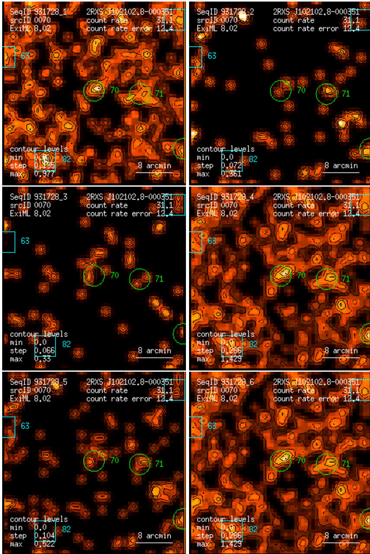
Figure 70: RASS 931728: detection 0070: band rate images, Gaussian filter: (1) PSPC channels 11 – 41, (2) 52 – 90, (3) 91 – 201, (4) 11 – 235, (5) 52 – 201, (6) 11 – 201. Broad band rates in counts/ks. Band rate contour levels in counts/ks/arcmin 2 .
