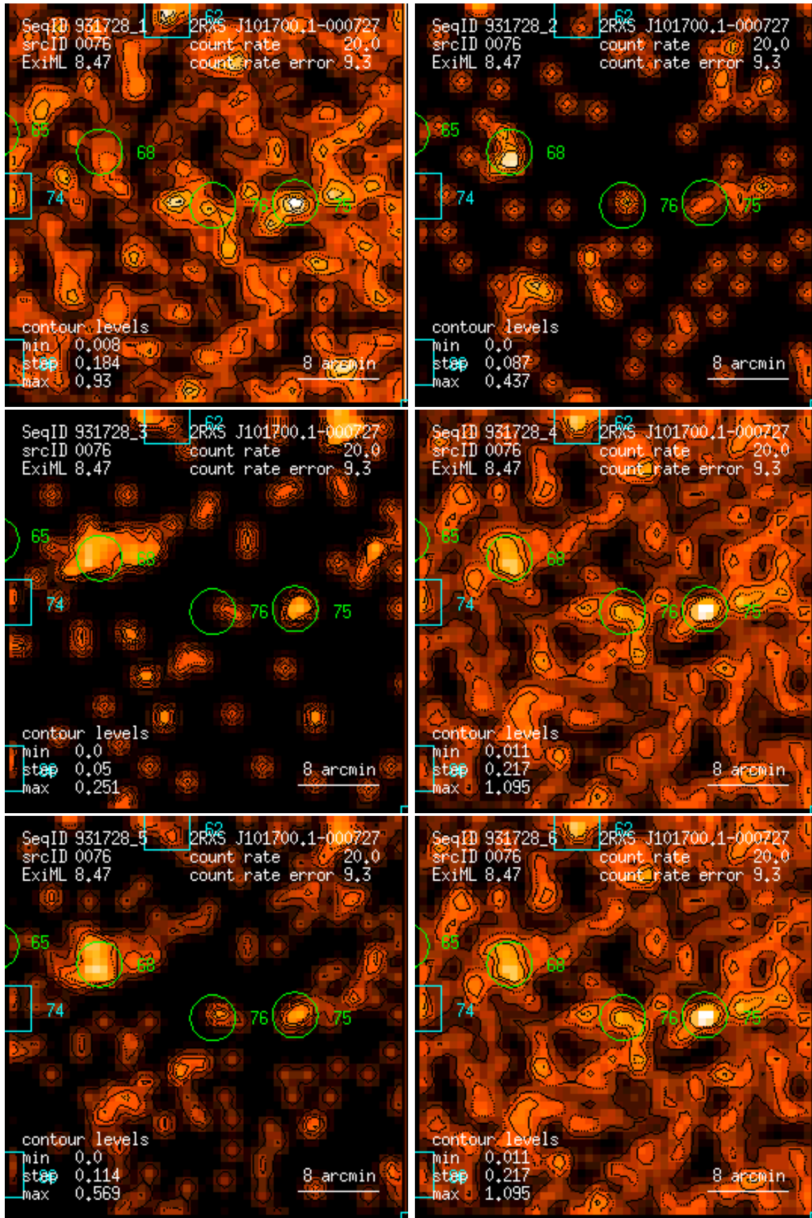
Figure 76: RASS 931728: detection 0076: band rate images, Gaussian filter: (1) PSPC channels 11 – 41, (2) 52 – 90, (3) 91 – 201, (4) 11 – 235, (5) 52 – 201, (6) 11 – 201. Broad band rates in counts/ks. Band rate contour levels in counts/ks/arcmin 2 .
