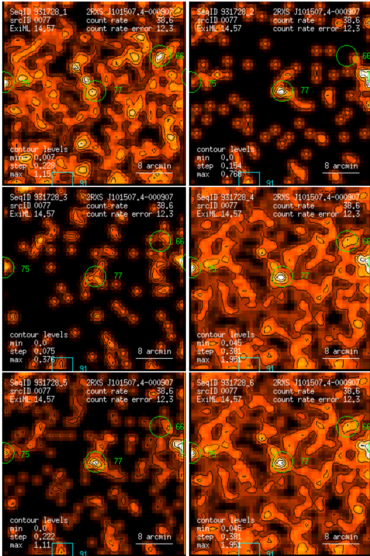
Figure 77: RASS 931728: detection 0077: band rate images, Gaussian filter: (1) PSPC channels 11 – 41, (2) 52 – 90, (3) 91 – 201, (4) 11 – 235, (5) 52 – 201, (6) 11 – 201. Broad band rates in counts/ks. Band rate contour levels in counts/ks/arcmin 2 .
