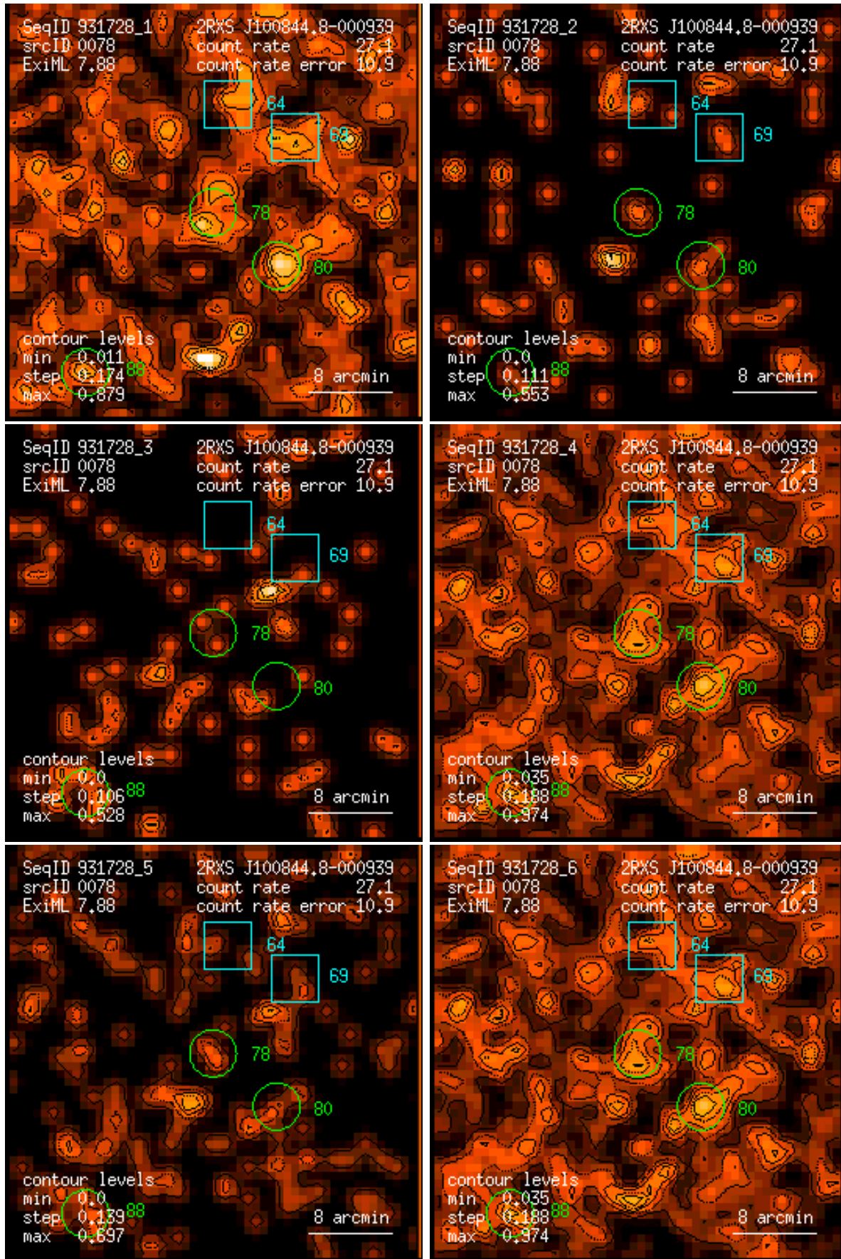
Figure 78: RASS 931728: detection 0078: band rate images, Gaussian filter: (1) PSPC channels 11 – 41, (2) 52 – 90, (3) 91 – 201, (4) 11 – 235, (5) 52 – 201, (6) 11 – 201. Broad band rates in counts/ks. Band rate contour levels in counts/ks/arcmin 2 .
