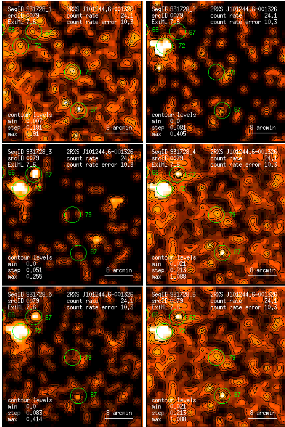
Figure 79: RASS 931728: detection 0079: band rate images, Gaussian filter: (1) PSPC channels 11 – 41, (2) 52 – 90, (3) 91 – 201, (4) 11 – 235, (5) 52 – 201, (6) 11 – 201. Broad band rates in counts/ks. Band rate contour levels in counts/ks/arcmin 2 .
