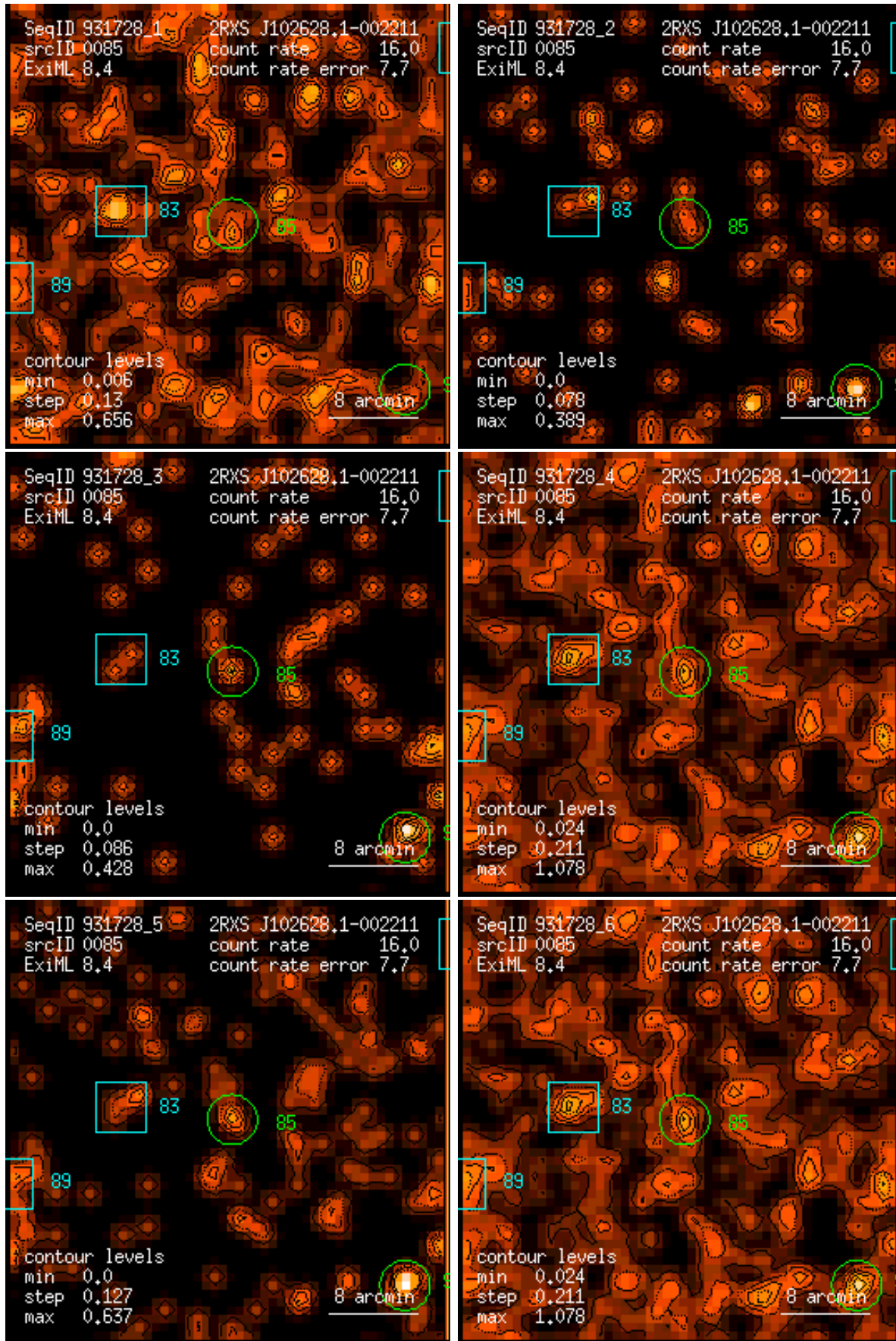
Figure 85: RASS 931728: detection 0085: band rate images, Gaussian filter: (1) PSPC channels 11 – 41, (2) 52 – 90, (3) 91 – 201, (4) 11 – 235, (5) 52 – 201, (6) 11 – 201. Broad band rates in counts/ks. Band rate contour levels in counts/ks/arcmin 2 .
