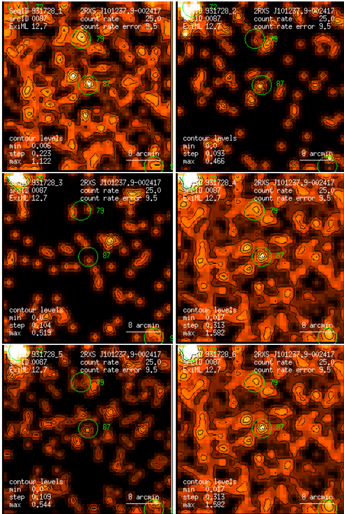
Figure 87: RASS 931728: detection 0087: band rate images, Gaussian filter: (1) PSPC channels 11 – 41, (2) 52 – 90, (3) 91 – 201, (4) 11 – 235, (5) 52 – 201, (6) 11 – 201. Broad band rates in counts/ks. Band rate contour levels in counts/ks/arcmin 2 .
