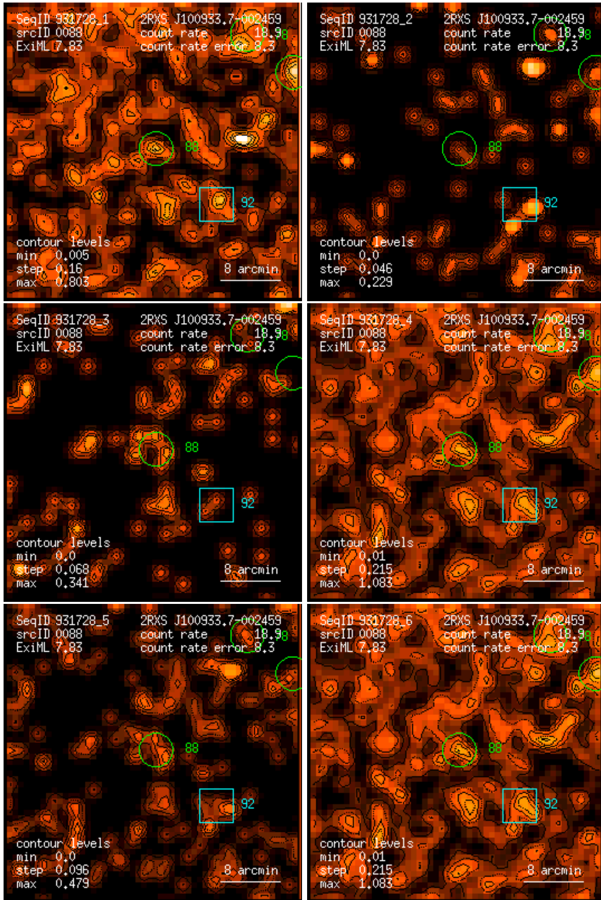
Figure 88: RASS 931728: detection 0088: band rate images, Gaussian filter: (1) PSPC channels 11 – 41, (2) 52 – 90, (3) 91 – 201, (4) 11 – 235, (5) 52 – 201, (6) 11 – 201. Broad band rates in counts/ks. Band rate contour levels in counts/ks/arcmin 2 .
