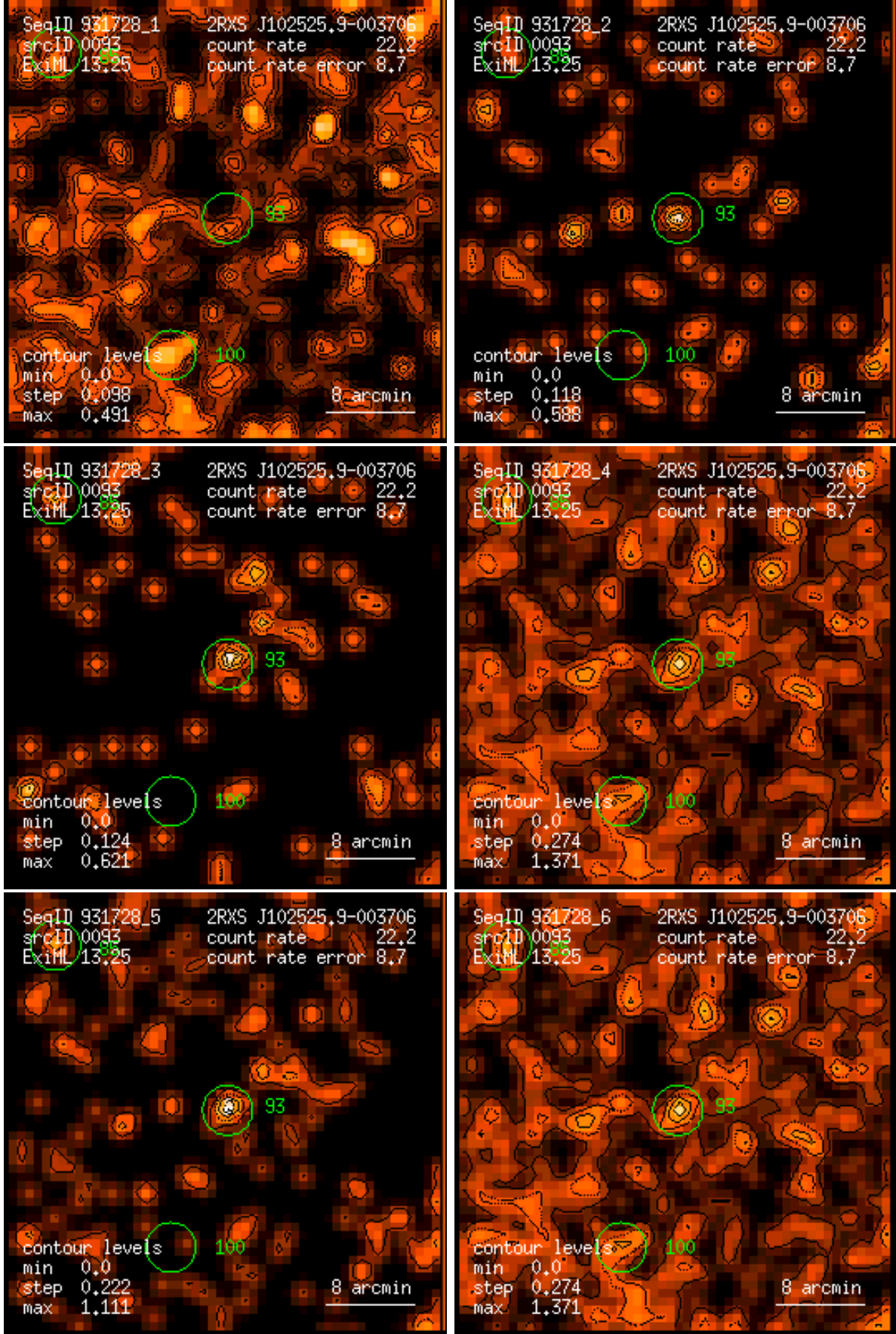
Figure 93: RASS 931728: detection 0093: band rate images, Gaussian filter: (1) PSPC channels 11 – 41, (2) 52 – 90, (3) 91 – 201, (4) 11 – 235, (5) 52 – 201, (6) 11 – 201. Broad band rates in counts/ks. Band rate contour levels in counts/ks/arcmin 2 .
