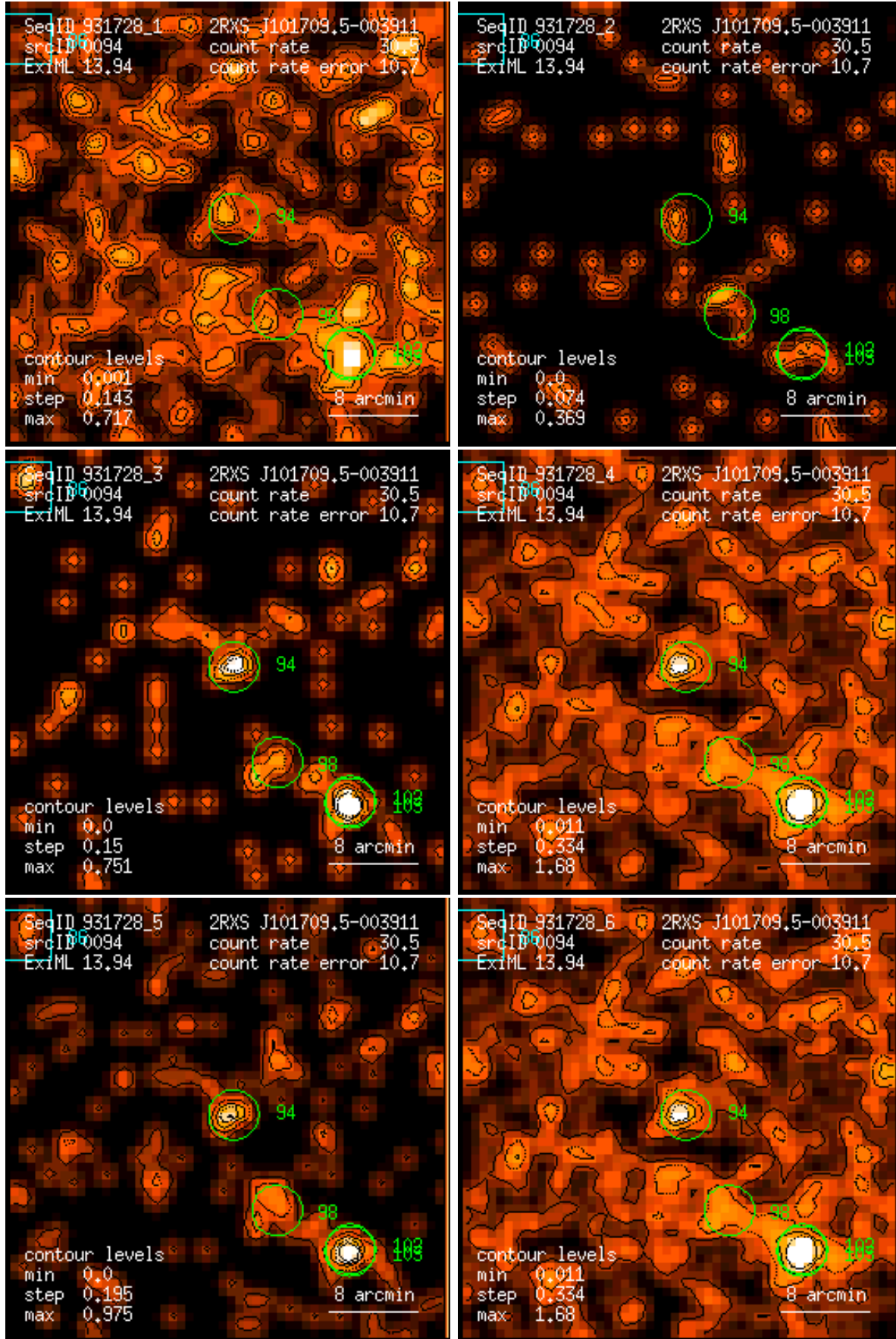
Figure 94: RASS 931728: detection 0094: band rate images, Gaussian filter: (1) PSPC channels 11 – 41, (2) 52 – 90, (3) 91 – 201, (4) 11 – 235, (5) 52 – 201, (6) 11 – 201. Broad band rates in counts/ks. Band rate contour levels in counts/ks/arcmin 2 .
