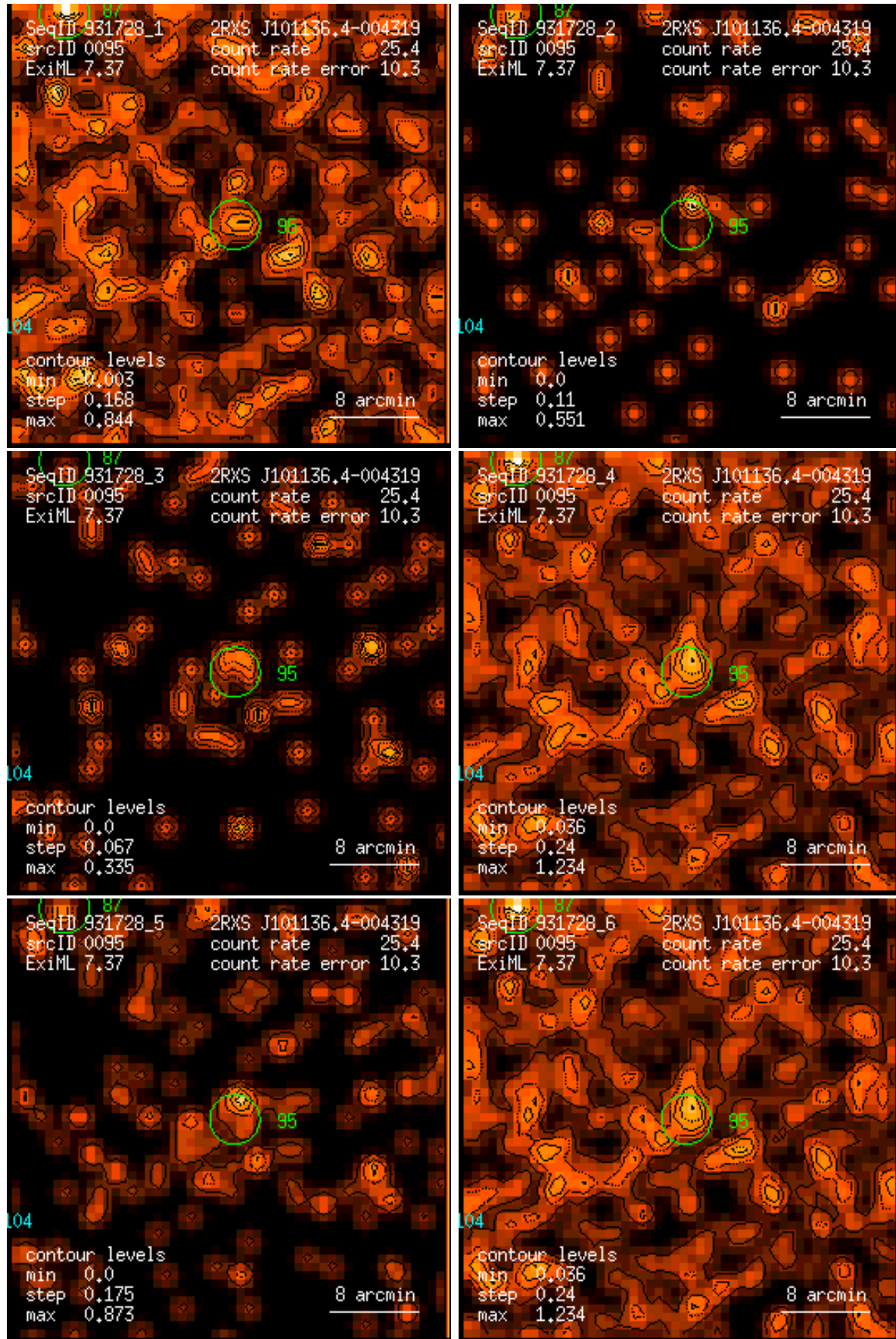
Figure 95: RASS 931728: detection 0095: band rate images, Gaussian filter: (1) PSPC channels 11 – 41, (2) 52 – 90, (3) 91 – 201, (4) 11 – 235, (5) 52 – 201, (6) 11 – 201. Broad band rates in counts/ks. Band rate contour levels in counts/ks/arcmin 2 .
