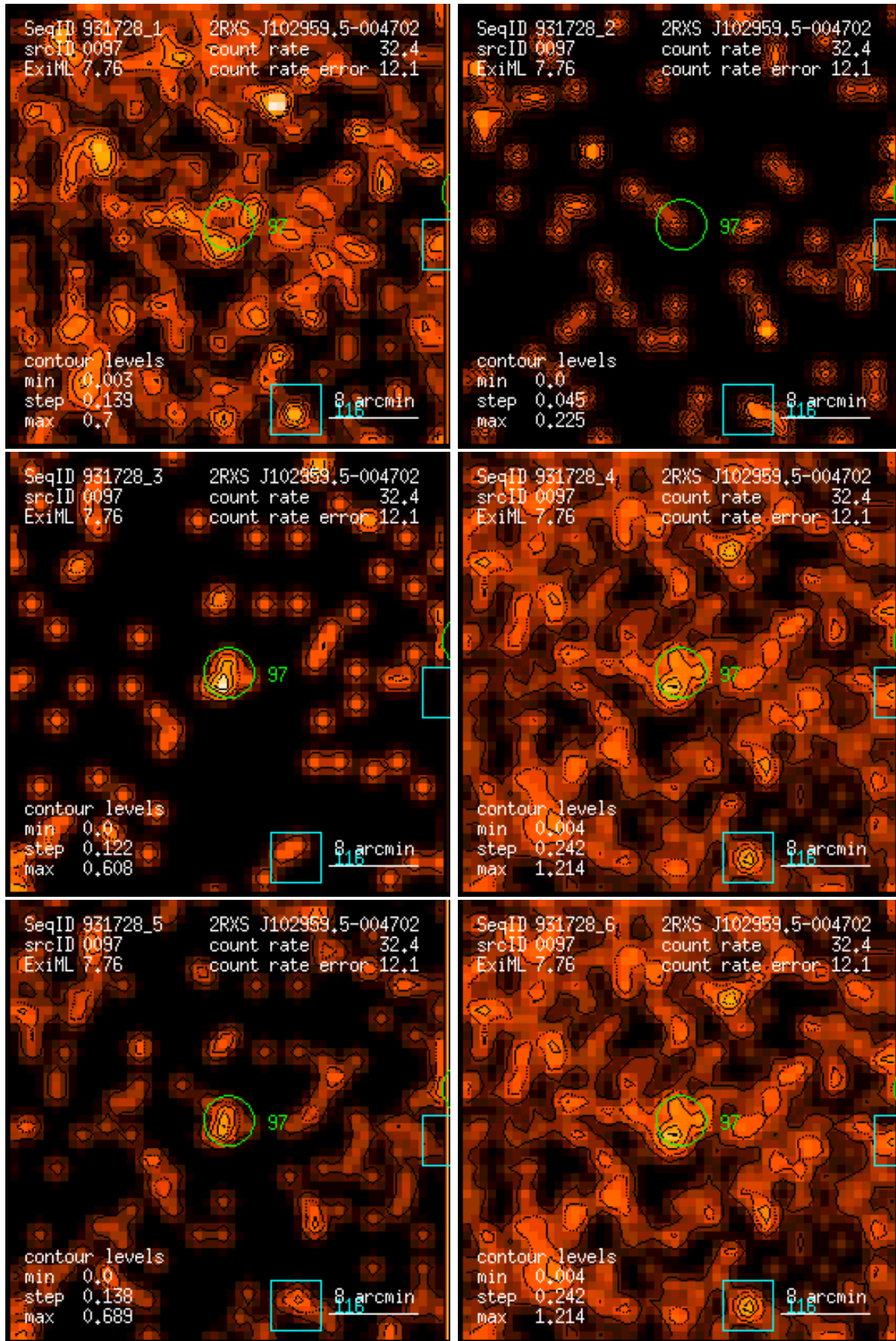
Figure 97: RASS 931728: detection 0097: band rate images, Gaussian filter: (1) PSPC channels 11 – 41, (2) 52 – 90, (3) 91 – 201, (4) 11 – 235, (5) 52 – 201, (6) 11 – 201. Broad band rates in counts/ks. Band rate contour levels in counts/ks/arcmin 2 .
