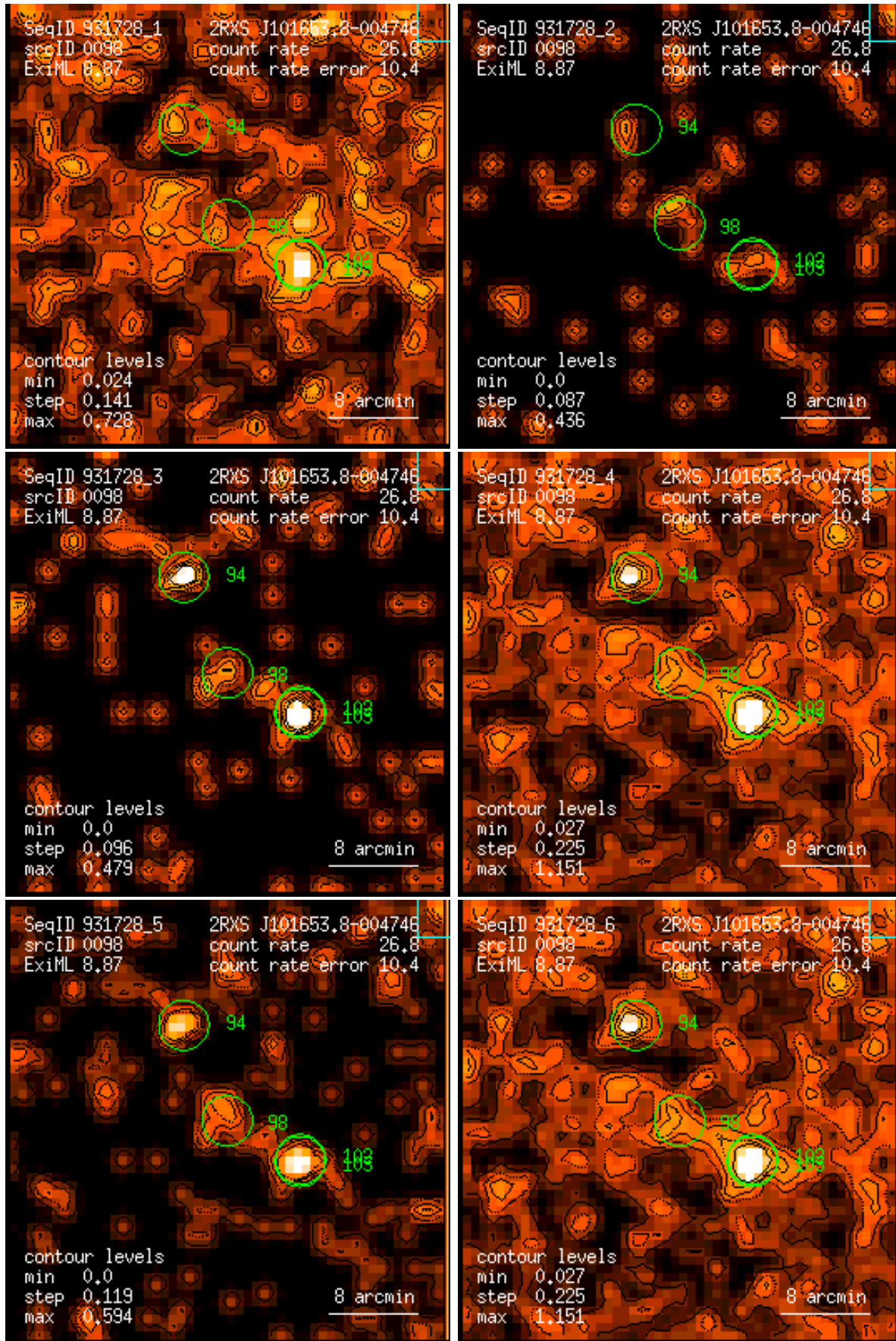
Figure 98: RASS 931728: detection 0098: band rate images, Gaussian filter: (1) PSPC channels 11 – 41, (2) 52 – 90, (3) 91 – 201, (4) 11 – 235, (5) 52 – 201, (6) 11 – 201. Broad band rates in counts/ks. Band rate contour levels in counts/ks/arcmin 2 .
