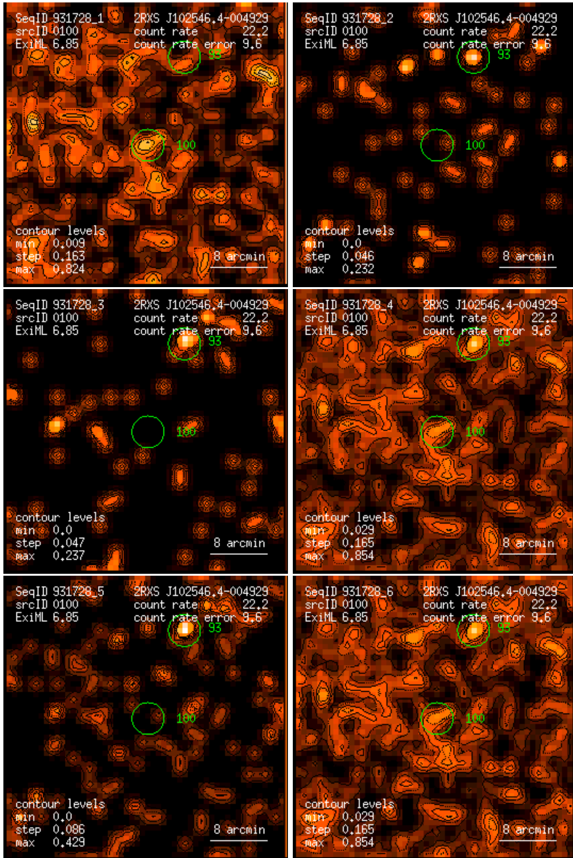
Figure 100: RASS 931728: detection 0100: band rate images, Gaussian filter: (1) PSPC channels 11 – 41, (2) 52 – 90, (3) 91 – 201, (4) 11 – 235, (5) 52 – 201, (6) 11 – 201. Broad band rates in counts/ks. Band rate contour levels in counts/ks/arcmin 2 .
