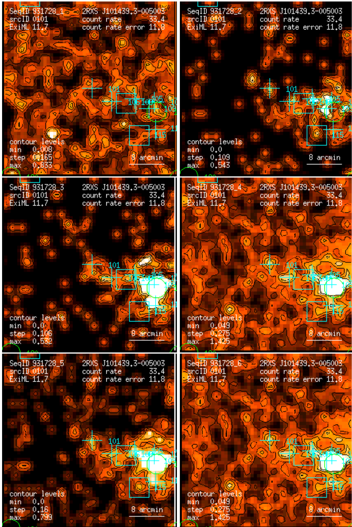
Figure 101: RASS 931728: detection 0101: band rate images, Gaussian filter: (1) PSPC channels 11 – 41, (2) 52 – 90, (3) 91 – 201, (4) 11 – 235, (5) 52 – 201, (6) 11 – 201. Broad band rates in counts/ks. Band rate contour levels in counts/ks/arcmin 2 .
