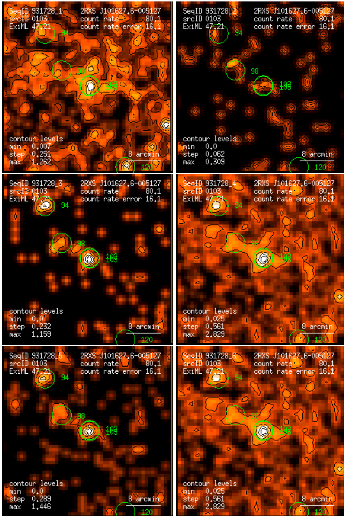
Figure 103: RASS 931728: detection 0103: band rate images, Gaussian filter: (1) PSPC channels 11 – 41, (2) 52 – 90, (3) 91 – 201, (4) 11 – 235, (5) 52 – 201, (6) 11 – 201. Broad band rates in counts/ks. Band rate contour levels in counts/ks/arcmin 2 .
