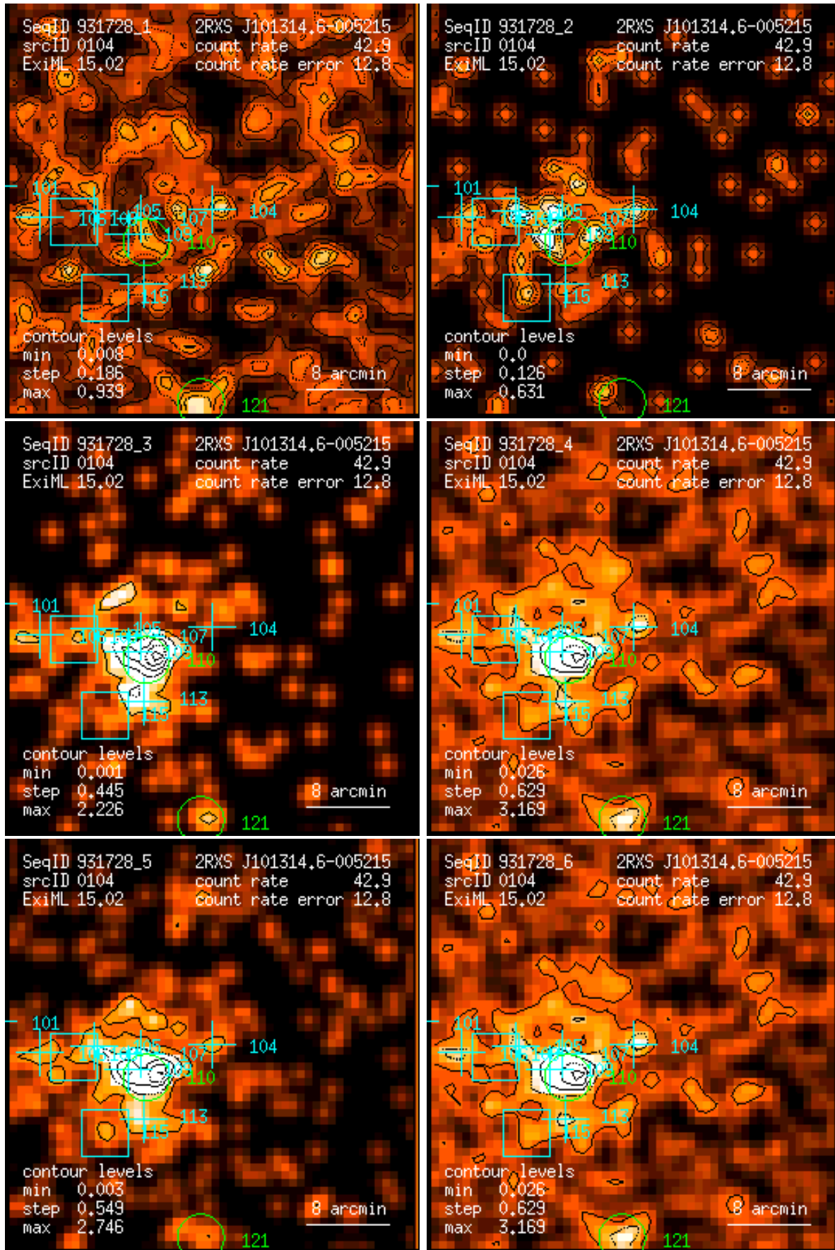
Figure 104: RASS 931728: detection 0104: band rate images, Gaussian filter: (1) PSPC channels 11 – 41, (2) 52 – 90, (3) 91 – 201, (4) 11 – 235, (5) 52 – 201, (6) 11 – 201. Broad band rates in counts/ks. Band rate contour levels in counts/ks/arcmin 2 .
