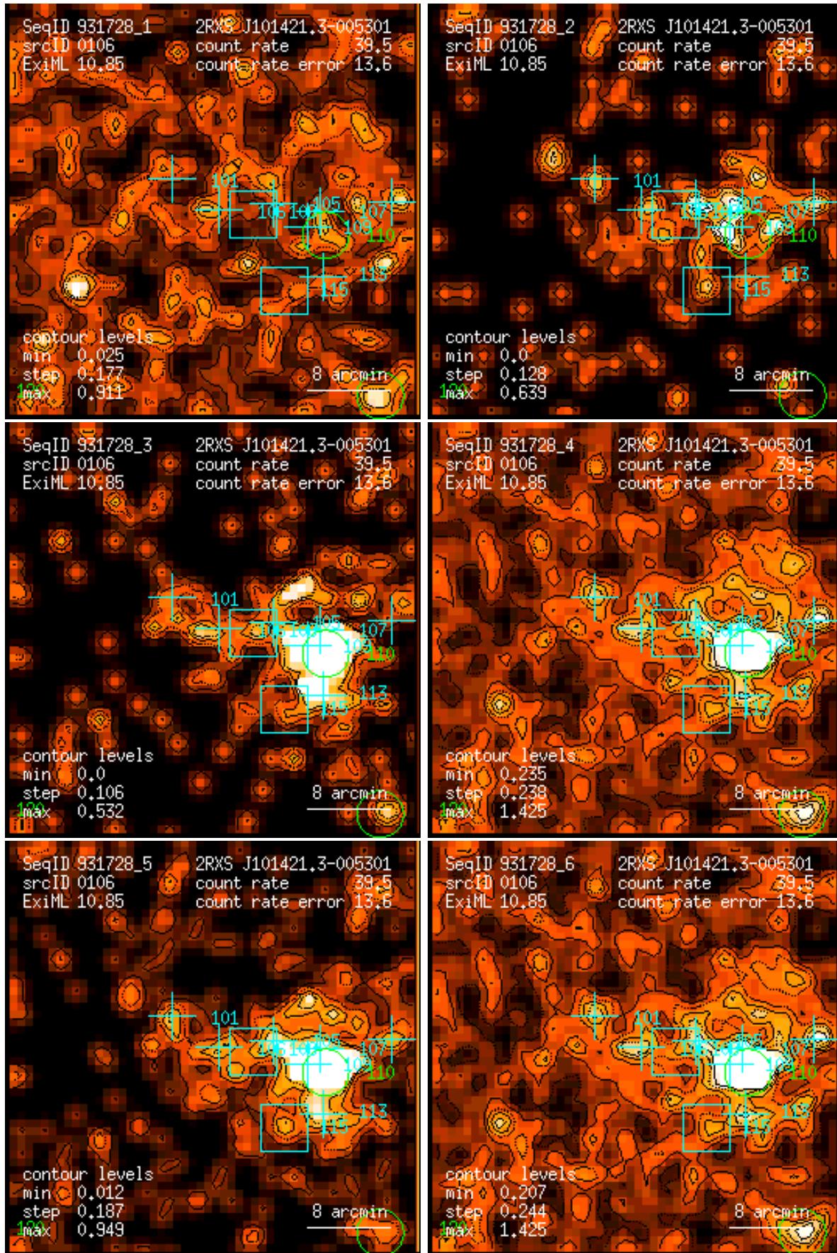
Figure 106: RASS 931728: detection 0106: band rate images, Gaussian filter: (1) PSPC channels 11 – 41, (2) 52 – 90, (3) 91 – 201, (4) 11 – 235, (5) 52 – 201, (6) 11 – 201. Broad band rates in counts/ks. Band rate contour levels in counts/ks/arcmin 2 .
