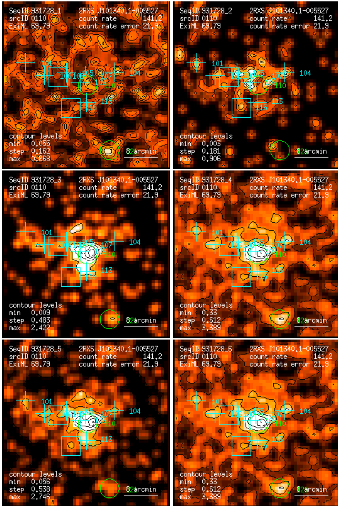
Figure 110: RASS 931728: detection 0110: band rate images, Gaussian filter: (1) PSPC channels 11 – 41, (2) 52 – 90, (3) 91 – 201, (4) 11 – 235, (5) 52 – 201, (6) 11 – 201. Broad band rates in counts/ks. Band rate contour levels in counts/ks/arcmin 2 .
