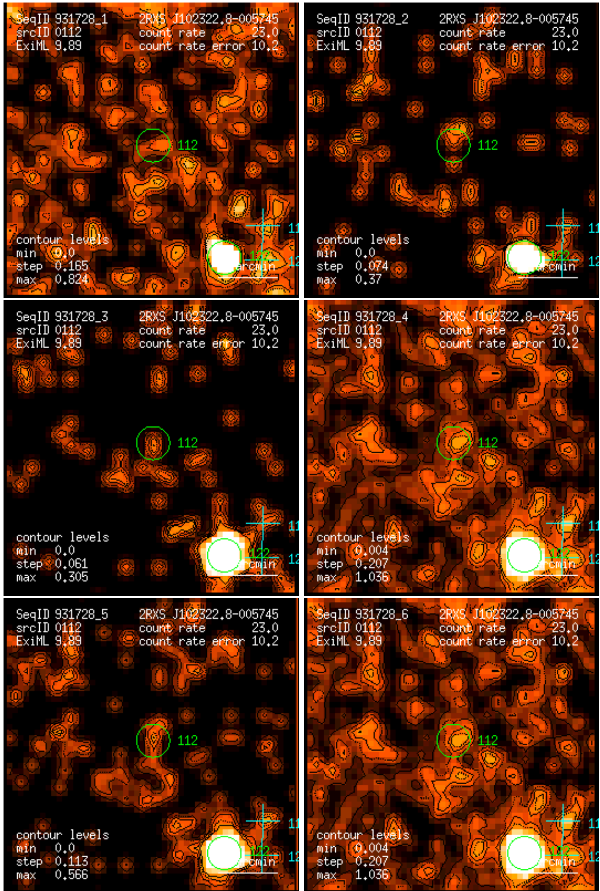
Figure 112: RASS 931728: detection 0112: band rate images, Gaussian filter: (1) PSPC channels 11 – 41, (2) 52 – 90, (3) 91 – 201, (4) 11 – 235, (5) 52 – 201, (6) 11 – 201. Broad band rates in counts/ks. Band rate contour levels in counts/ks/arcmin 2 .
