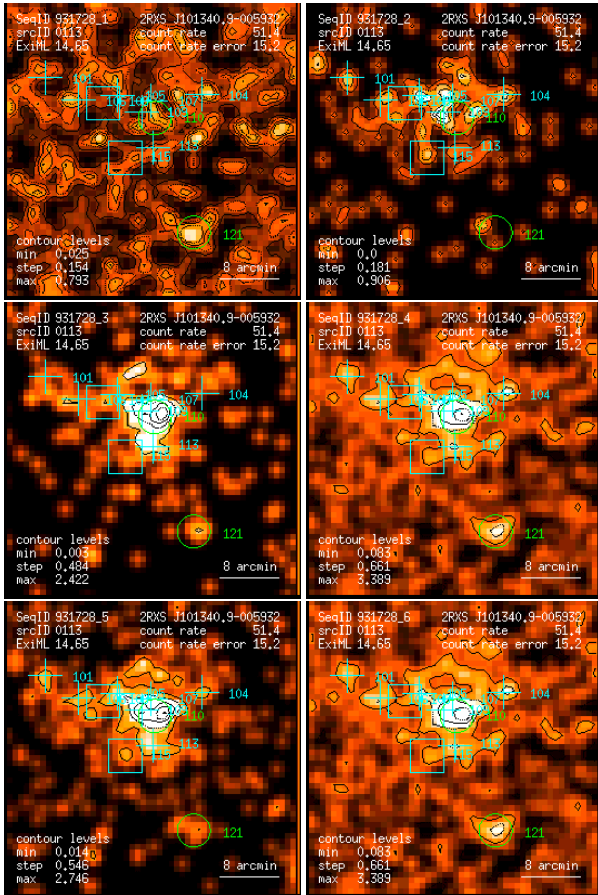
Figure 113: RASS 931728: detection 0113: band rate images, Gaussian filter: (1) PSPC channels 11 – 41, (2) 52 – 90, (3) 91 – 201, (4) 11 – 235, (5) 52 – 201, (6) 11 – 201. Broad band rates in counts/ks. Band rate contour levels in counts/ks/arcmin 2 .
