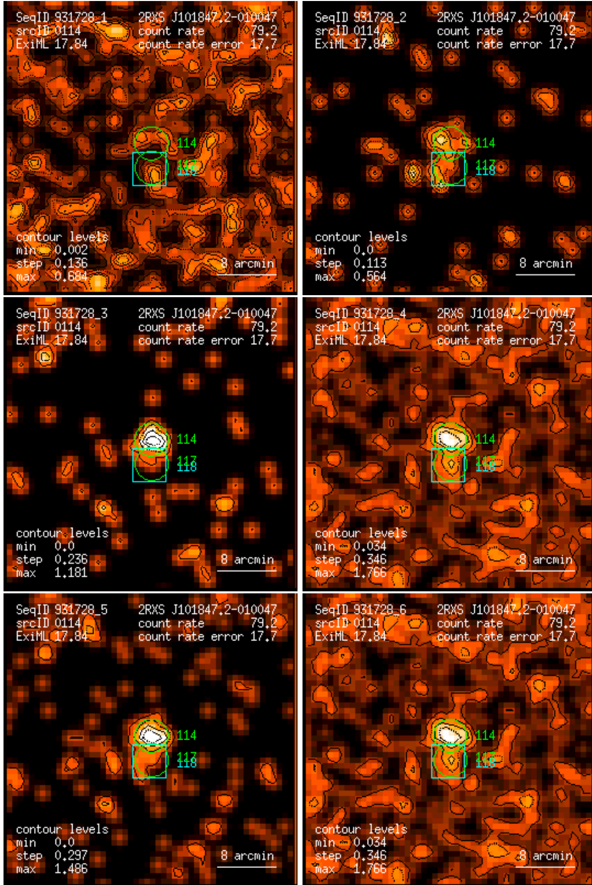
Figure 114: RASS 931728: detection 0114: band rate images, Gaussian filter: (1) PSPC channels 11 – 41, (2) 52 – 90, (3) 91 – 201, (4) 11 – 235, (5) 52 – 201, (6) 11 – 201. Broad band rates in counts/ks. Band rate contour levels in counts/ks/arcmin 2 .
