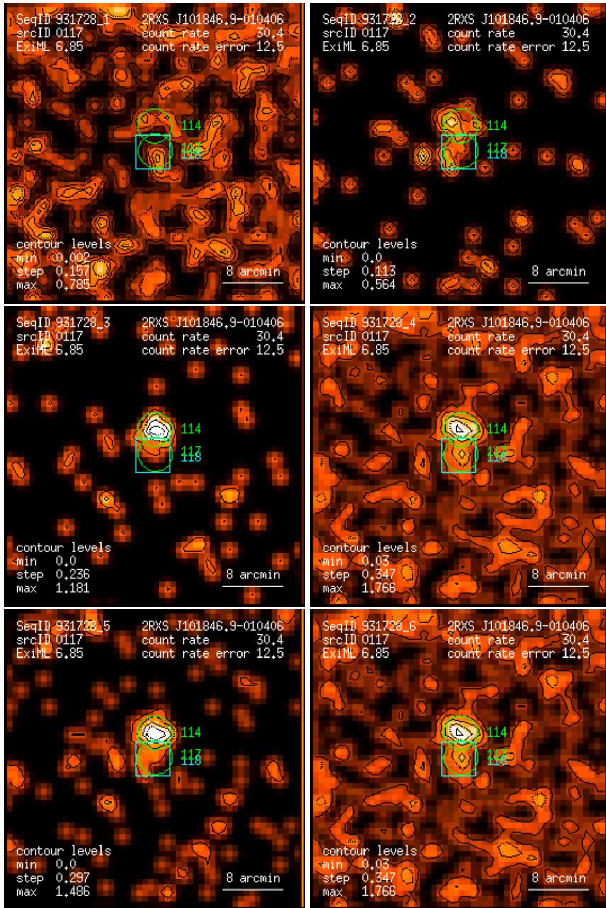
Figure 117: RASS 931728: detection 0117: band rate images, Gaussian filter: (1) PSPC channels 11 – 41, (2) 52 – 90, (3) 91 – 201, (4) 11 – 235, (5) 52 – 201, (6) 11 – 201. Broad band rates in counts/ks. Band rate contour levels in counts/ks/arcmin 2 .
