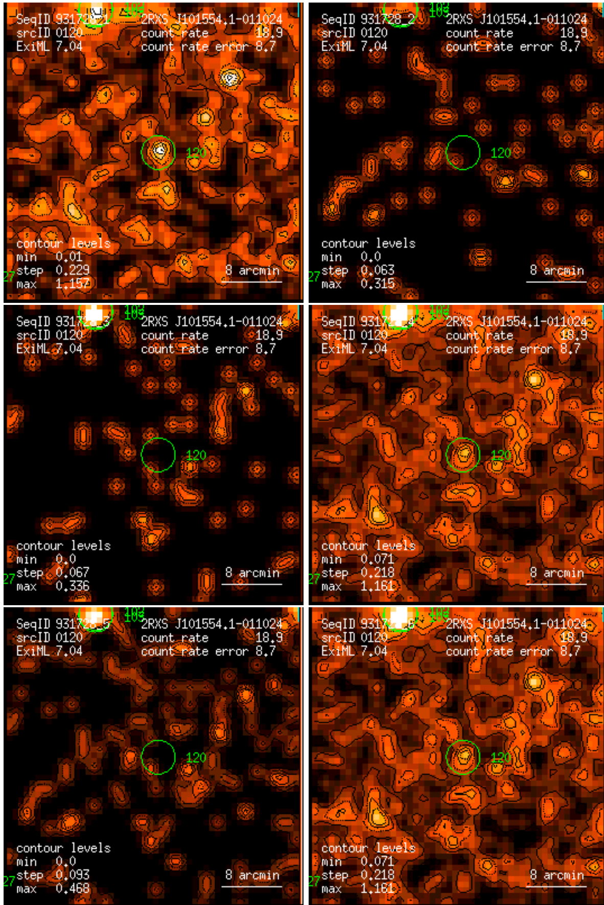
Figure 120: RASS 931728: detection 0120: band rate images, Gaussian filter: (1) PSPC channels 11 – 41, (2) 52 – 90, (3) 91 – 201, (4) 11 – 235, (5) 52 – 201, (6) 11 – 201. Broad band rates in counts/ks. Band rate contour levels in counts/ks/arcmin 2 .
