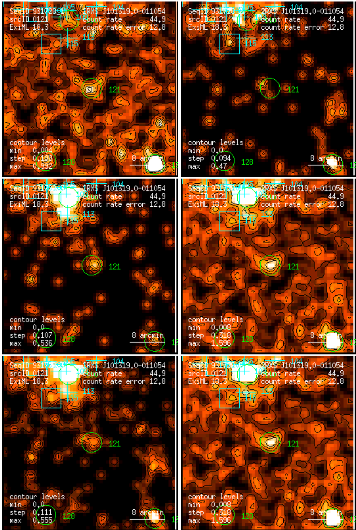
Figure 121: RASS 931728: detection 0121: band rate images, Gaussian filter: (1) PSPC channels 11 – 41, (2) 52 – 90, (3) 91 – 201, (4) 11 – 235, (5) 52 – 201, (6) 11 – 201. Broad band rates in counts/ks. Band rate contour levels in counts/ks/arcmin 2 .
