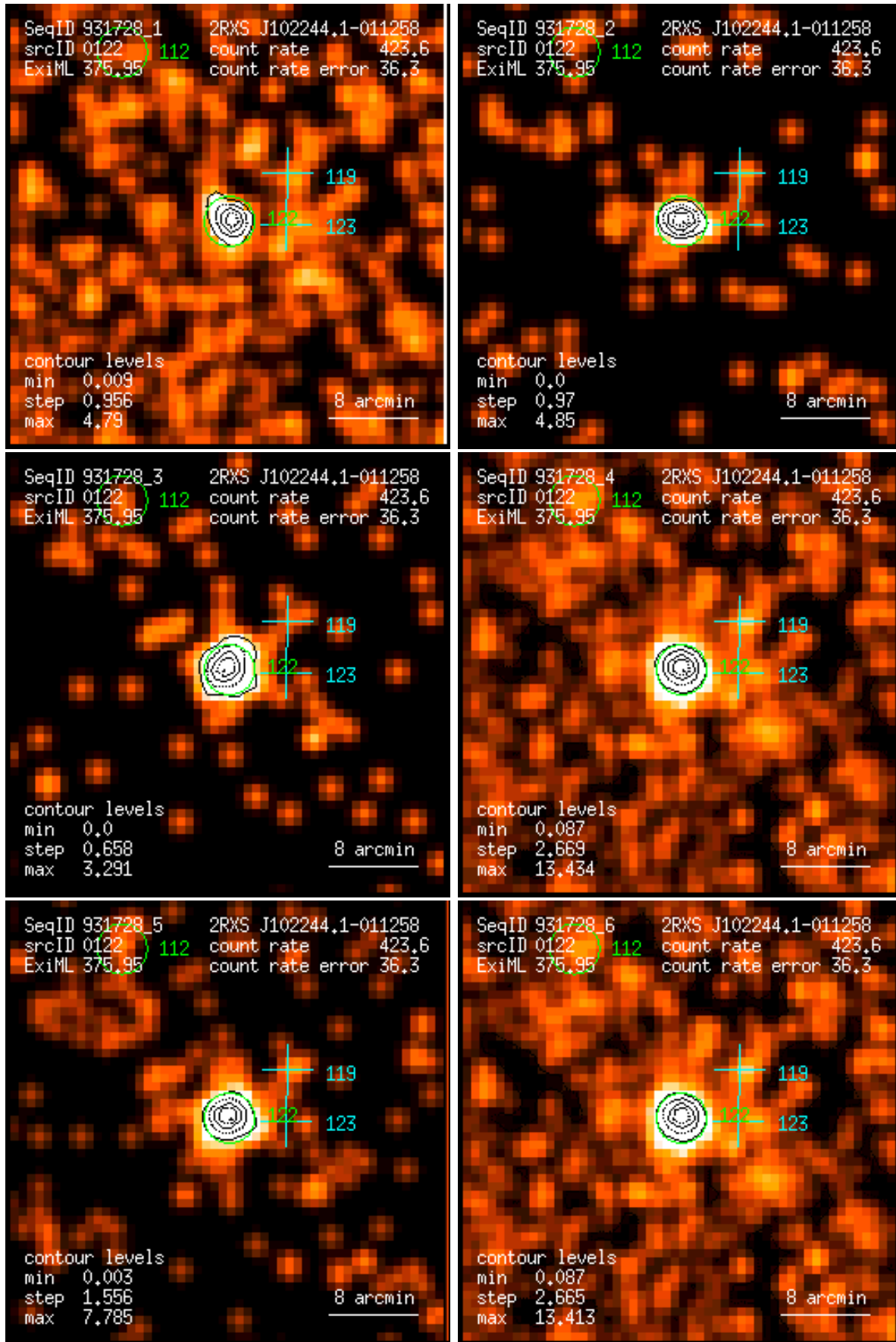
Figure 122: RASS 931728: detection 0122: band rate images, Gaussian filter: (1) PSPC channels 11 – 41, (2) 52 – 90, (3) 91 – 201, (4) 11 – 235, (5) 52 – 201, (6) 11 – 201. Broad band rates in counts/ks. Band rate contour levels in counts/ks/arcmin 2 .
