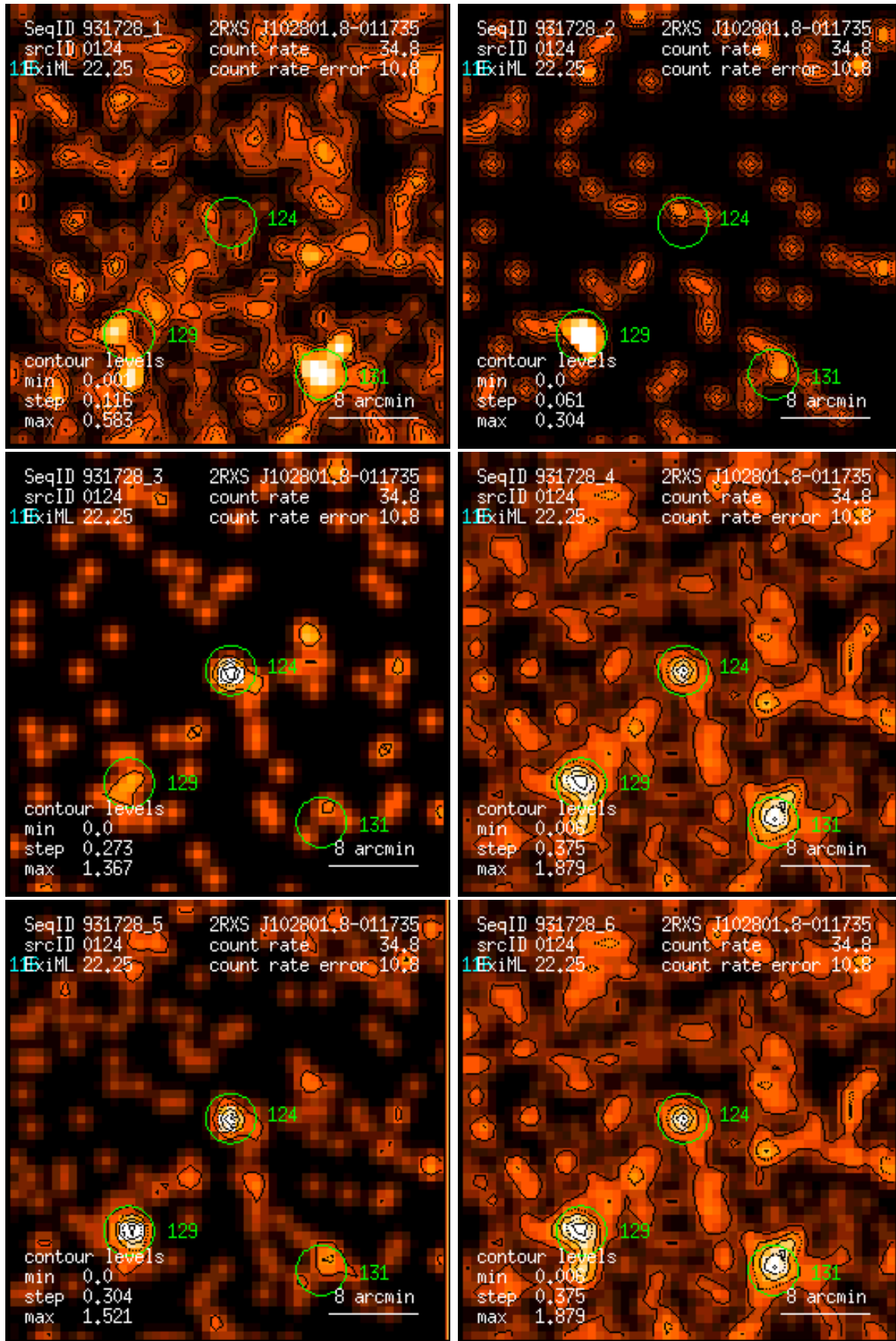
Figure 124: RASS 931728: detection 0124: band rate images, Gaussian filter: (1) PSPC channels 11 – 41, (2) 52 – 90, (3) 91 – 201, (4) 11 – 235, (5) 52 – 201, (6) 11 – 201. Broad band rates in counts/ks. Band rate contour levels in counts/ks/arcmin 2 .
