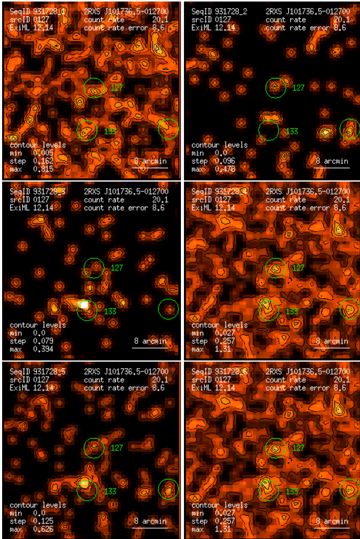
Figure 127: RASS 931728: detection 0127: band rate images, Gaussian filter: (1) PSPC channels 11 – 41, (2) 52 – 90, (3) 91 – 201, (4) 11 – 235, (5) 52 – 201, (6) 11 – 201. Broad band rates in counts/ks. Band rate contour levels in counts/ks/arcmin 2 .
