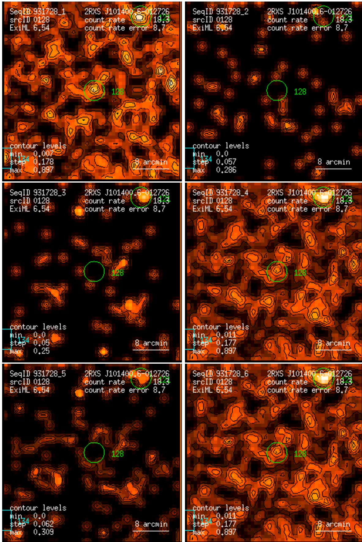
Figure 128: RASS 931728: detection 0128: band rate images, Gaussian filter: (1) PSPC channels 11 – 41, (2) 52 – 90, (3) 91 – 201, (4) 11 – 235, (5) 52 – 201, (6) 11 – 201. Broad band rates in counts/ks. Band rate contour levels in counts/ks/arcmin 2 .
