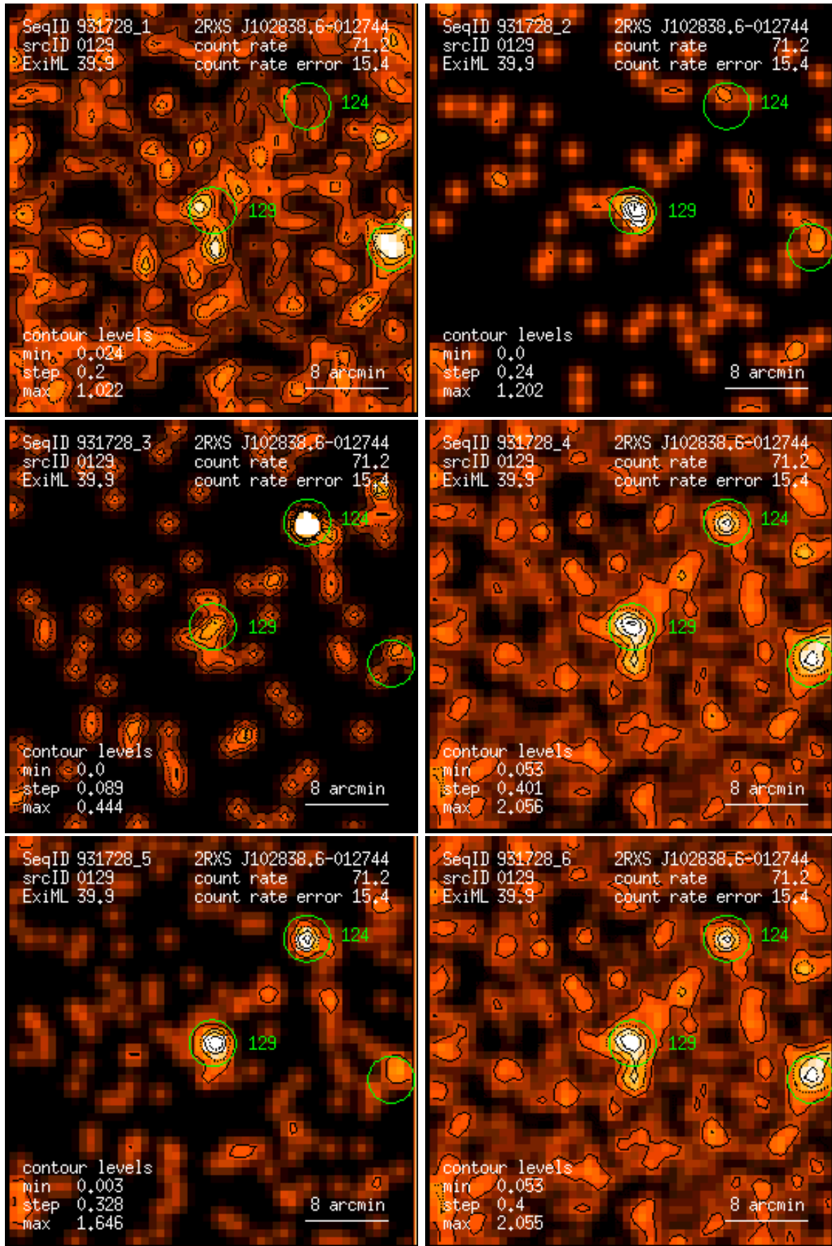
Figure 129: RASS 931728: detection 0129: band rate images, Gaussian filter: (1) PSPC channels 11 – 41, (2) 52 – 90, (3) 91 – 201, (4) 11 – 235, (5) 52 – 201, (6) 11 – 201. Broad band rates in counts/ks. Band rate contour levels in counts/ks/arcmin 2 .
