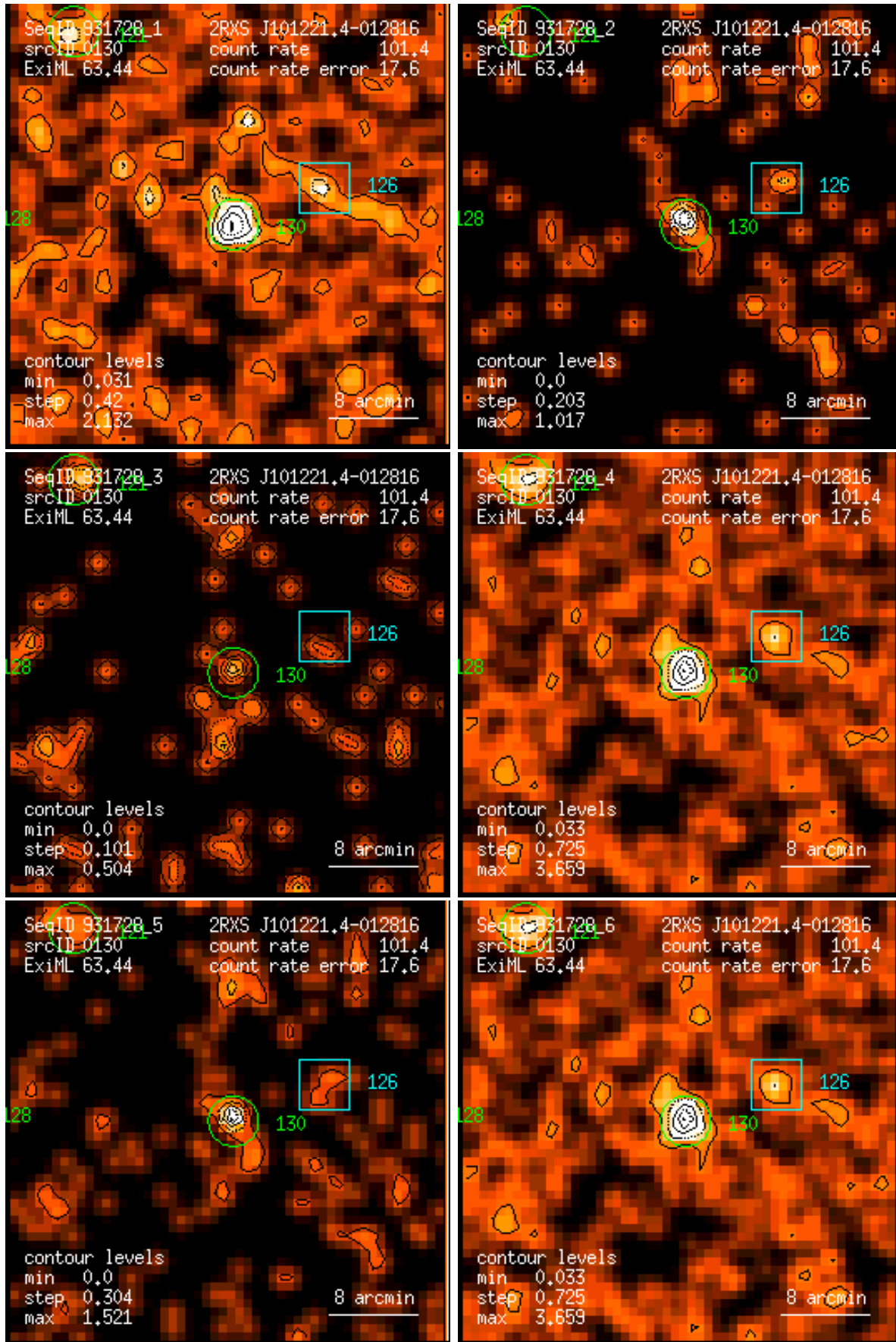
Figure 130: RASS 931728: detection 0130: band rate images, Gaussian filter: (1) PSPC channels 11 – 41, (2) 52 – 90, (3) 91 – 201, (4) 11 – 235, (5) 52 – 201, (6) 11 – 201. Broad band rates in counts/ks. Band rate contour levels in counts/ks/arcmin 2 .
