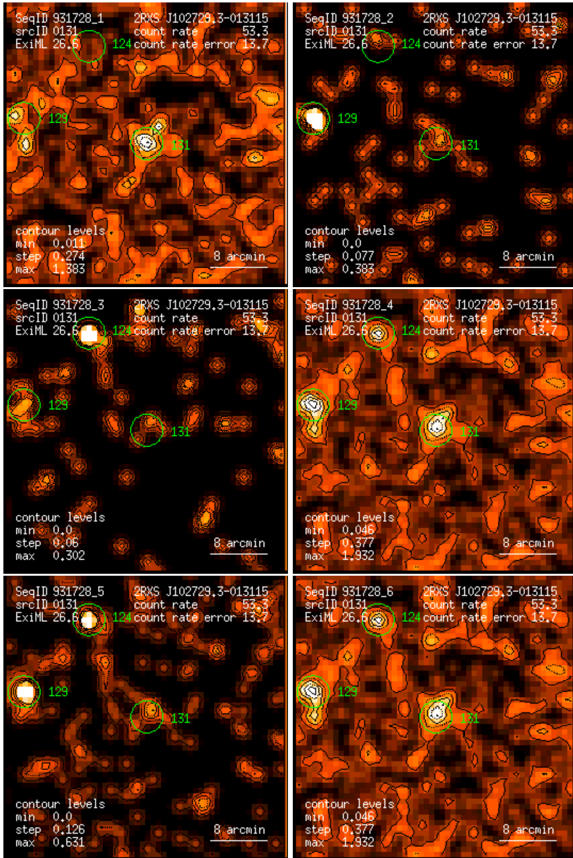
Figure 131: RASS 931728: detection 0131: band rate images, Gaussian filter: (1) PSPC channels 11 – 41, (2) 52 – 90, (3) 91 – 201, (4) 11 – 235, (5) 52 – 201, (6) 11 – 201. Broad band rates in counts/ks. Band rate contour levels in counts/ks/arcmin 2 .
