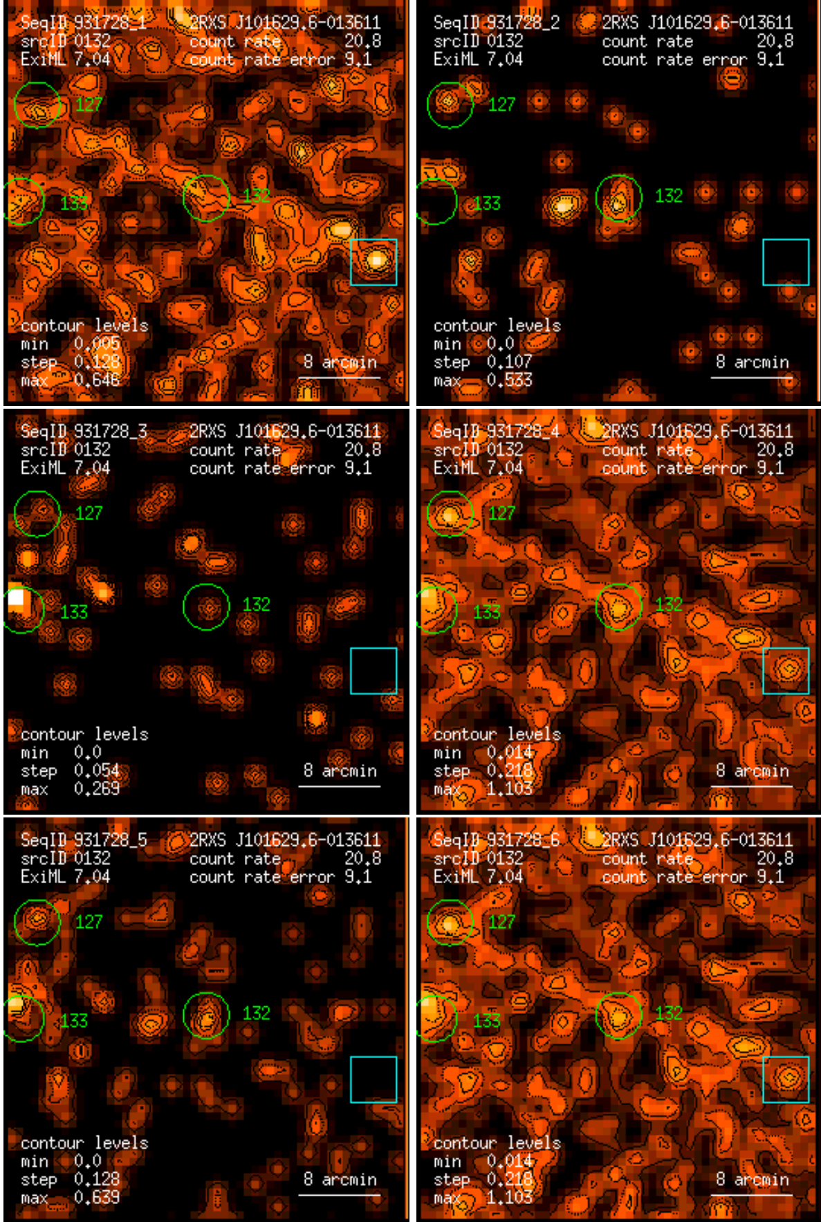
Figure 132: RASS 931728: detection 0132: band rate images, Gaussian filter: (1) PSPC channels 11 – 41, (2) 52 – 90, (3) 91 – 201, (4) 11 – 235, (5) 52 – 201, (6) 11 – 201. Broad band rates in counts/ks. Band rate contour levels in counts/ks/arcmin 2 .
