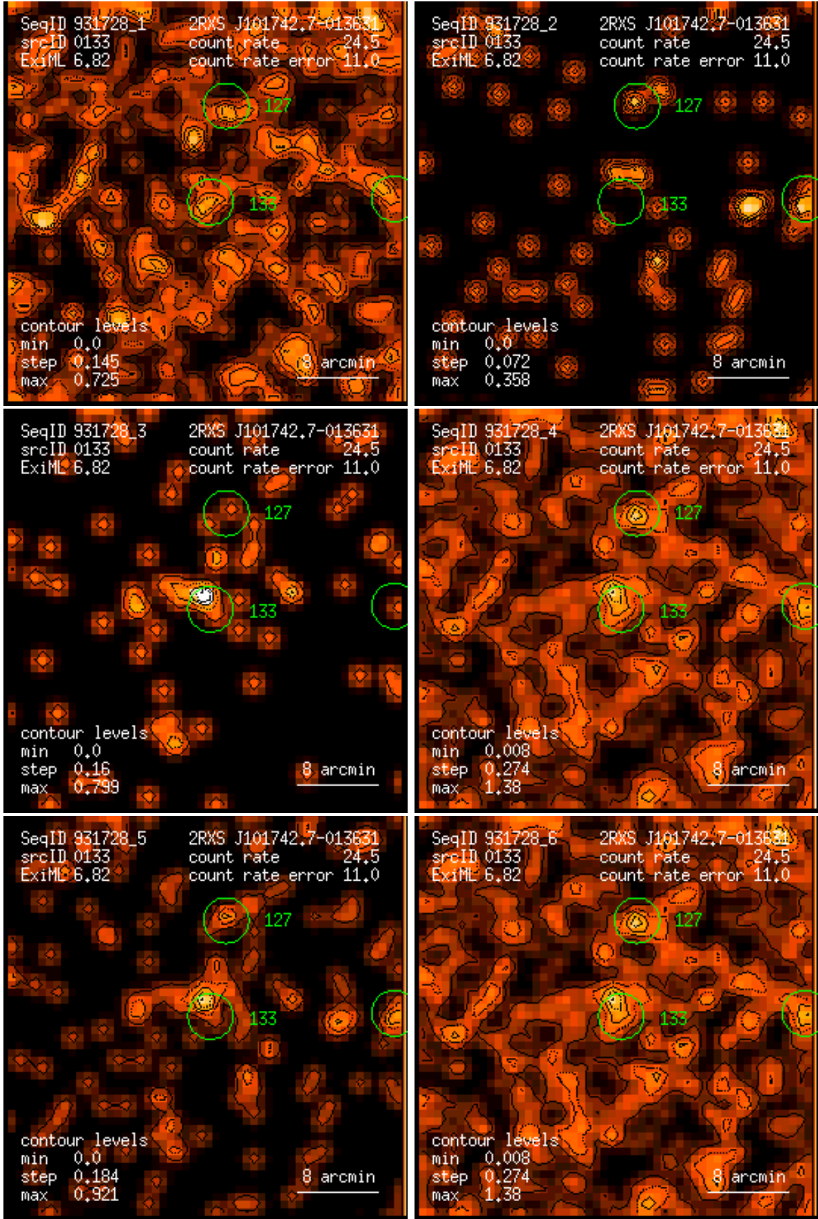
Figure 133: RASS 931728: detection 0133: band rate images, Gaussian filter: (1) PSPC channels 11 – 41, (2) 52 – 90, (3) 91 – 201, (4) 11 – 235, (5) 52 – 201, (6) 11 – 201. Broad band rates in counts/ks. Band rate contour levels in counts/ks/arcmin 2 .
