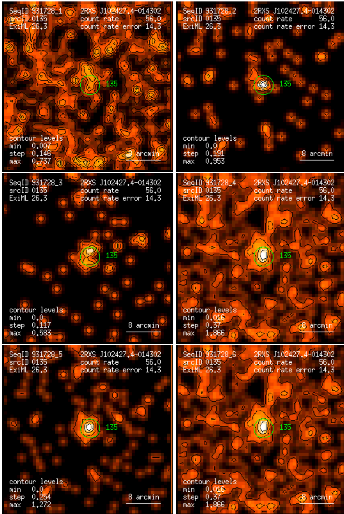
Figure 135: RASS 931728: detection 0135: band rate images, Gaussian filter: (1) PSPC channels 11 – 41, (2) 52 – 90, (3) 91 – 201, (4) 11 – 235, (5) 52 – 201, (6) 11 – 201. Broad band rates in counts/ks. Band rate contour levels in counts/ks/arcmin 2 .
