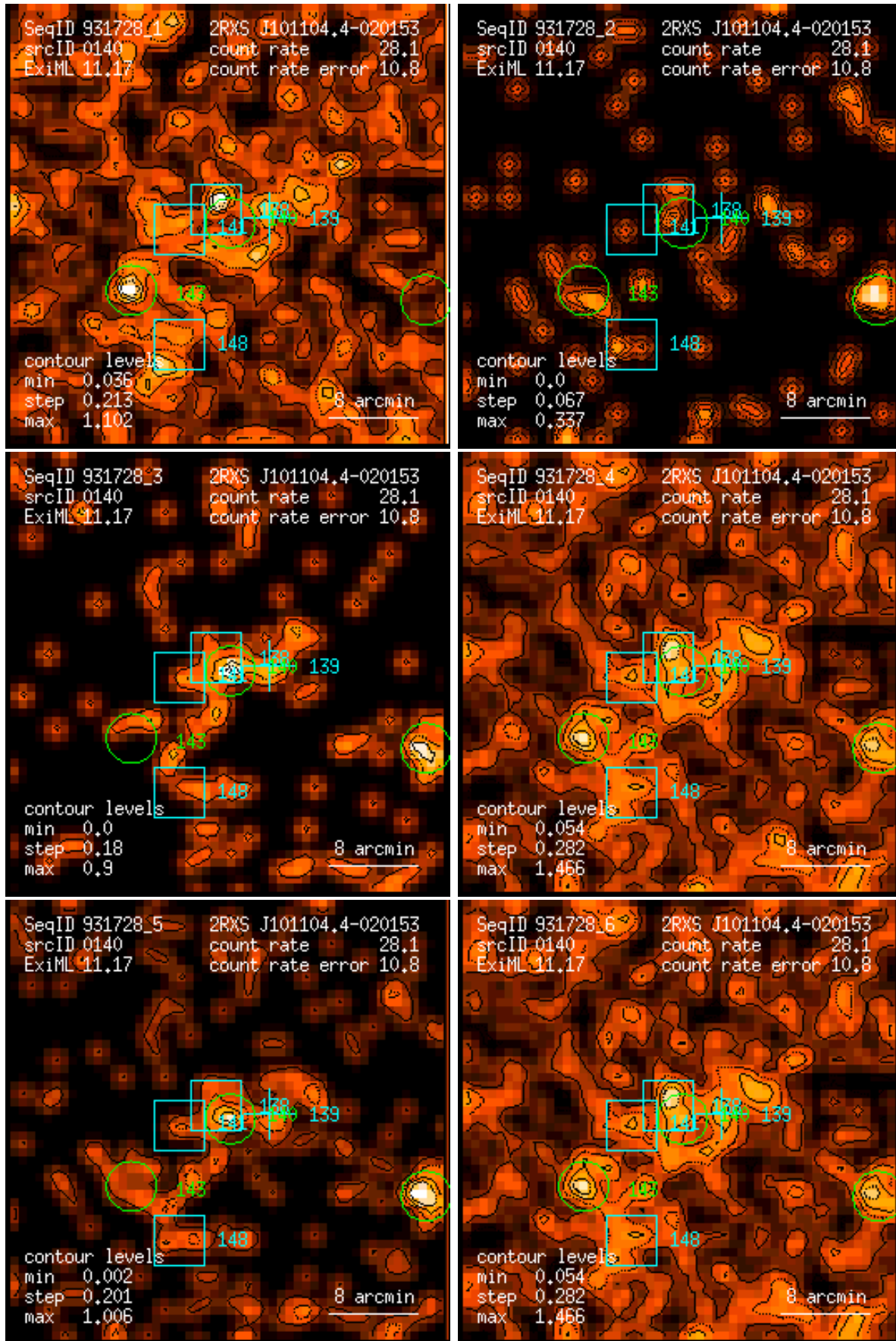
Figure 140: RASS 931728: detection 0140: band rate images, Gaussian filter: (1) PSPC channels 11 – 41, (2) 52 – 90, (3) 91 – 201, (4) 11 – 235, (5) 52 – 201, (6) 11 – 201. Broad band rates in counts/ks. Band rate contour levels in counts/ks/arcmin 2 .
